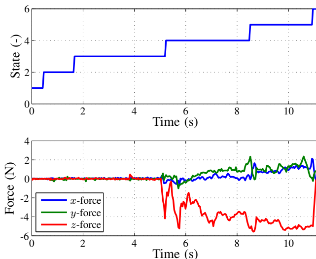
Fig. 7. Force data from an experiment, together with the state information. The x , y , and z forces are shown as blue, green, and red, respectively. The z -force is controlled to -5 (N) from state 4 and onwards. The threshold for activating the force control in the z -direction is set to -4 (N). The output in y - and x -directions are position controlled except in states 4 and 5, respectively, where they are velocity controlled.
