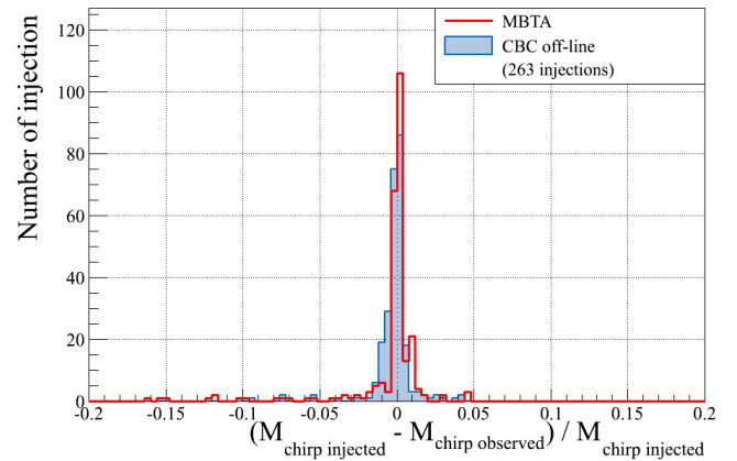
Fig. 7. This plot shows all the successful hardware injections which took place coherently in the three detectors. 93% of those which were above the threshold (expected SNR \geq 5.5 ) in each detector were detected in triple coincidence by MBTA.
