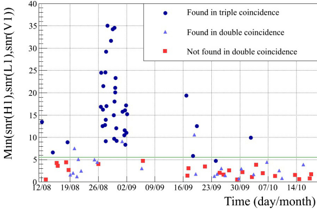
Fig. 7. This plot shows all the successful hardware injections which took place coherently in the three detectors. 93% of those which were above the threshold (expected SNR \geq 5.5 ) in each detector were detected in triple coincidence by MBTA.
