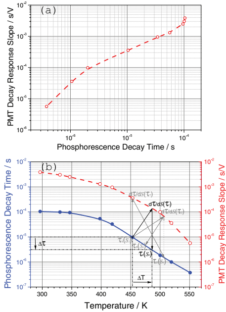
FIG. 8. PMT decay response slope for \text{La}_2\text{O}_2\text{S:Eu} (red circles) as a function of phosphorescence decay time (a) and as a function of temperature (b). The black arrows in graph (b) indicate how a measured decay time \tau_1(S_1) can be iteratively corrected towards \tau_r at reference signal output S_r ( < S_1 ) for which the phosphor was calibrated (blue dots).
