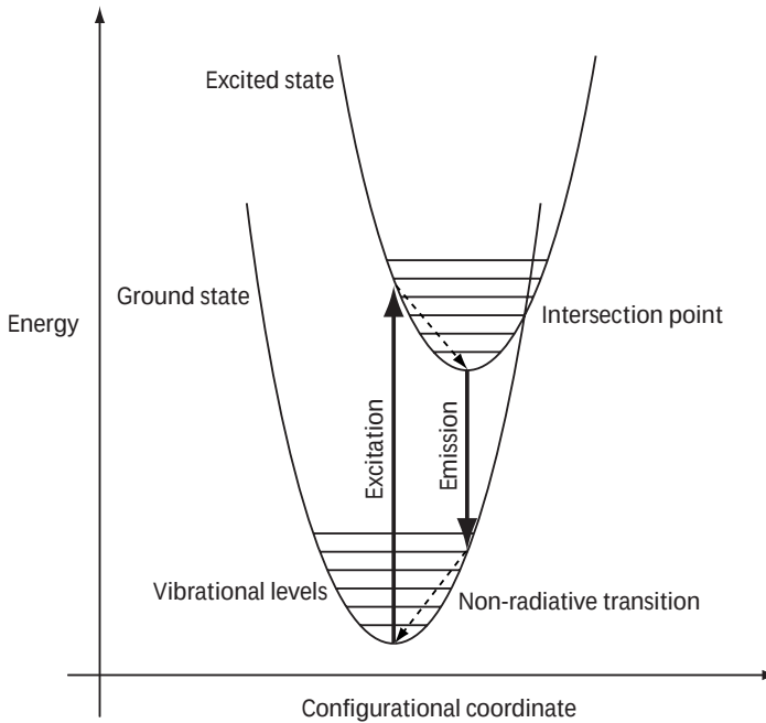
Figure 3.1 A configuration coordinate diagram
