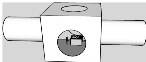
Figure 3. Schematic picture of the heated-grid reactor.
