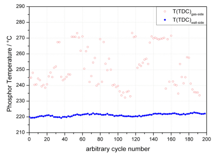
Figure 8. Single-shot phosphor temperatures at TDC during HCCI combustion, obtained for 100 consecutive cycles with the 59 \mu\text{m} phosphor coating.
