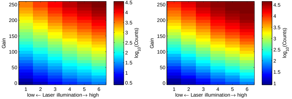
Figure 5.11 The mean signals in counts for the signals obtained through the IF456 filter (left) and the IF400 filter (right). Note that the count intensity scale is logarithmic.
