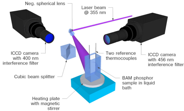
Figure 3. Experimental setup for the dual-camera experiment.
