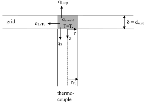
Figure A1. Geometry for a thermocouple attached on the surface of the grid.
