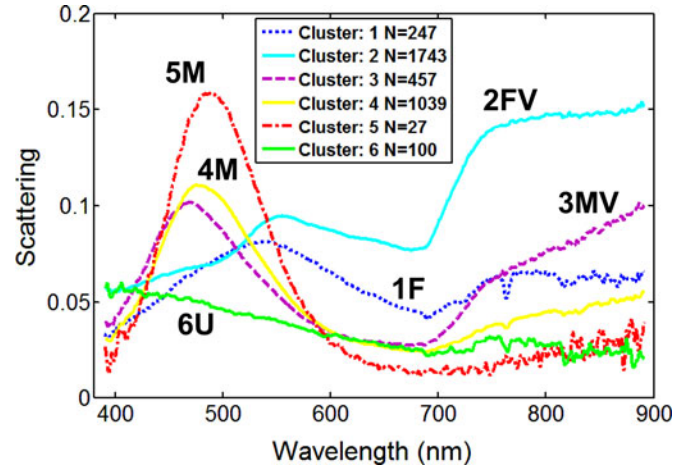
Fig. 7. Mean scattering spectra of each cluster. A scattering coefficient of 1 corresponds to the scatter from a white calibration polystyrene foam piece. M: male, F: female, V: vegetation imprint, U: uncertain. The spectra were interpreted as follows: 1F: female, 2FV: female with vegetation imprint, 3MV: male with vegetation imprint, 4M: male, 5M: male, 6U: uncertain.
