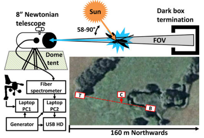
Fig. 2. Setup for the experiment. T: Newtonian telescope, C: calibration site, B: dark box termination. Light is collected by a 1-mm UV fiber in the focal plane of the telescope and fed to a compact spectrometer. Distance from the telescope to termination was 95 m of which the first 55 m covers the grassland and the remaining 40 m covers the river Klingavälsån.
