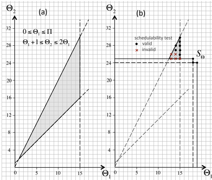
Figure 7. The example of a GMPR interface computation
