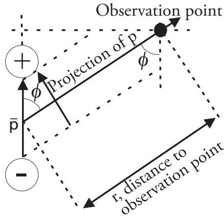
Figure 4.2 Illustration of the geometric relationship between polarization axis, \phi , observation point, and the projection of the polarization \bar{p} onto the plane facing the observation point.
