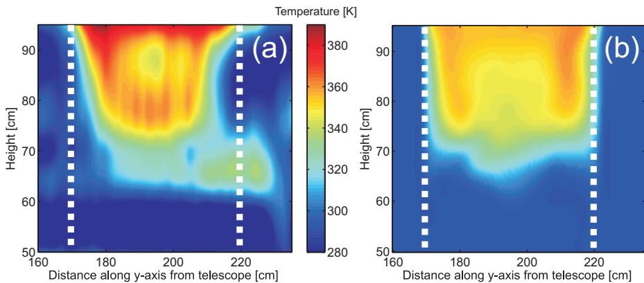
Figure 7.11 Temperature images of the y - z plane 6 cm outside the door measured with lidar is shown in (a), while (b) shows a simulated temperatures of a plane in the door way, i.e. 6 cm from the lidar plane.
