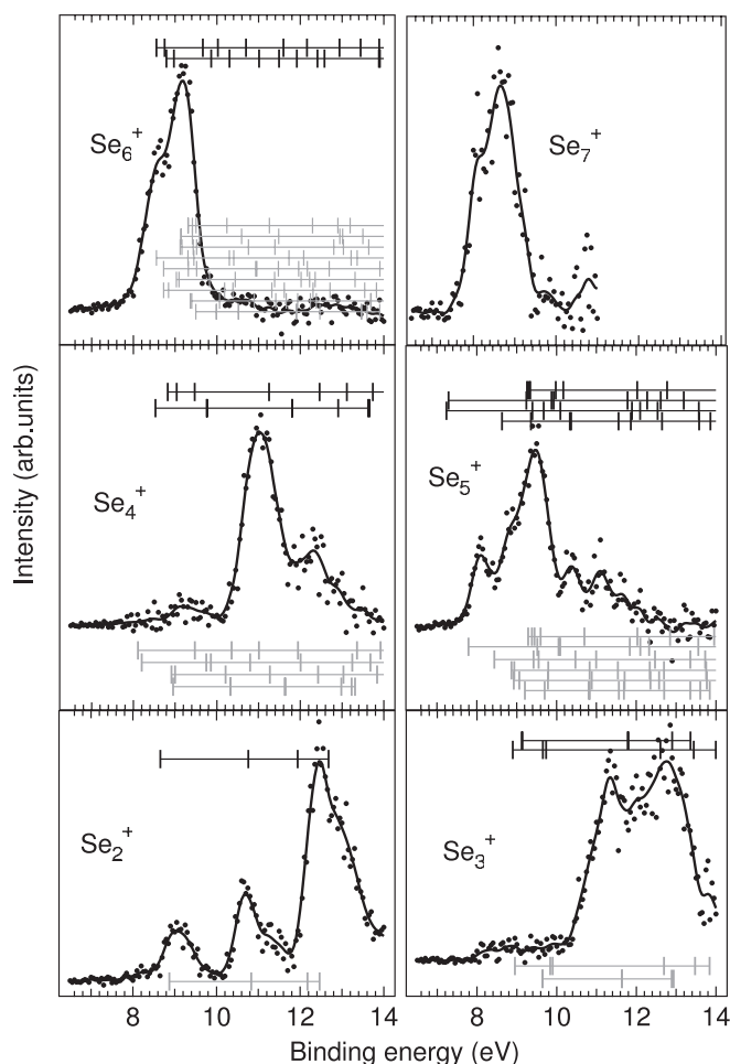
FIG. 4. The CIY spectra of \text{Se}_n clusters ( n = 2-7 ) measured at photon energy 22 \text{ eV} . The experimental data (black dots) are represented together with smoothed guide (solid) lines. The long horizontal bars present the total energy levels of isomers and every tiny vertical bar on a long bar stands for a molecular orbital (MO) energy level of corresponding cluster isomer. The calculation results of restricted open-shell Hartree-Fock theory (grey bars) are depicted below the corresponding CIY curve and the results of the unrestricted Hartree-Fock with second-order Møller-Plesset method (black bars) are given above the CIY spectrum. The maximum of counts (or coincidence events) 890 for \text{Se}_2 , 430 for \text{Se}_3 , 480 for \text{Se}_4 , 520 for \text{Se}_5 , 430 for \text{Se}_6 and 110 for \text{Se}_7 have been detected.
