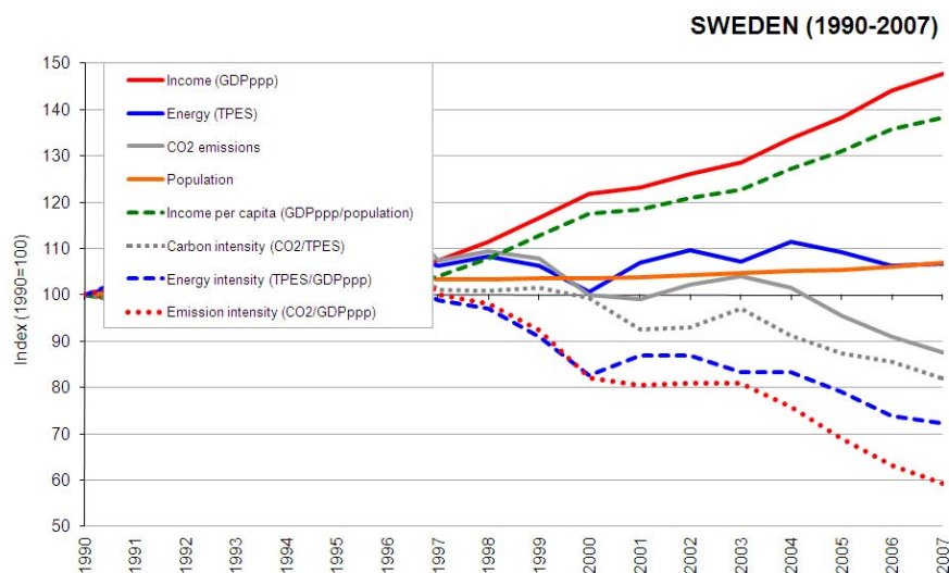
Figure 1: Estimated indicators for SWEDEN
