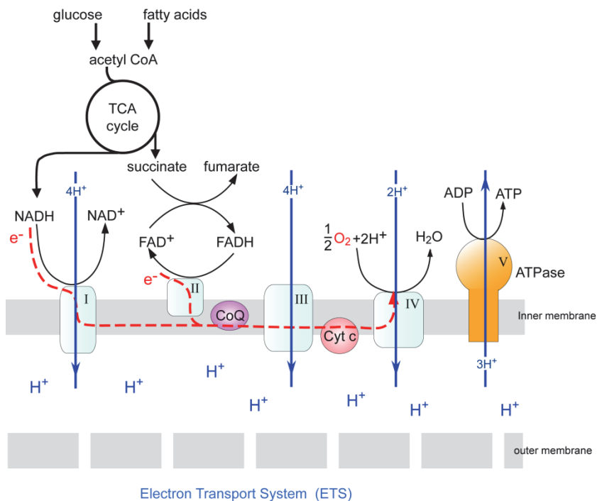
Fig.1 Schematic picture of ATP production by the mitochondrial respiratory system. Reproduced with permission from S. Morota.
