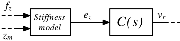
Figure 4.1 Block diagram for the closed-loop system with force feedback deflection compensation.
