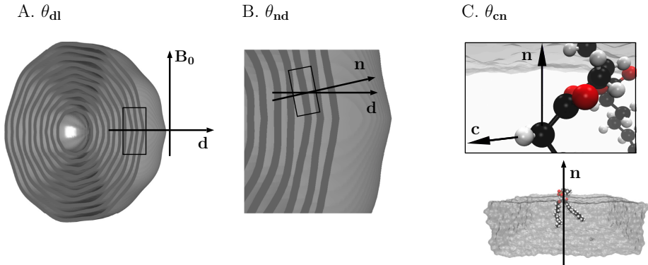
Figure 2.4: Illustration of the three angles that may be used to describe the orientation of C–H bonds in respect to a given laboratory frame axis \mathbf{l} . (A) \theta_{\mathbf{dl}} denotes the angle between the symmetry director axis \mathbf{d} of a liquid crystallite site and the fixed laboratory axis frame \mathbf{l} defined by the direction of the external magnetic field \mathbf{B}_0 . (B) \theta_{\mathbf{nd}} denotes the angle between a molecular frame axis with the direction of the bilayer normal \mathbf{n} and the symmetry director axis \mathbf{d} . (C) \theta_{\mathbf{cn}} represents the angle between the chemical bond principal axis of a given C–H pair and the bilayer normal \mathbf{n} . NMR order parameters S_{\mathbf{cl}} are time averages taken at short time intervals below 100 \mu\text{s} through which molecules diffuse slowly at restricted sites. During short times, around 10–100 ns, C–H bond reorientation is exclusively due to the variation of the angle \theta_{\mathbf{cn}} by means of fluctuations in C–C torsion angles and overall wobbling of the molecular segments. At longer time scales, variations of \theta_{\mathbf{nd}} due to lateral diffusion can also contribute to the time averaging of order parameters.
