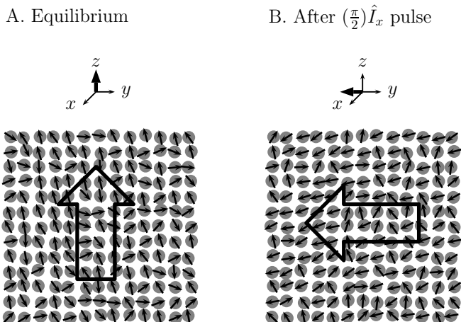
Figure 3.4: The effect of a 90^\circ RF pulse to an ensemble of spins as observed using a rotating frame. Usually RF pulses with time lengths around 1-10 \mu\text{s} are used.
