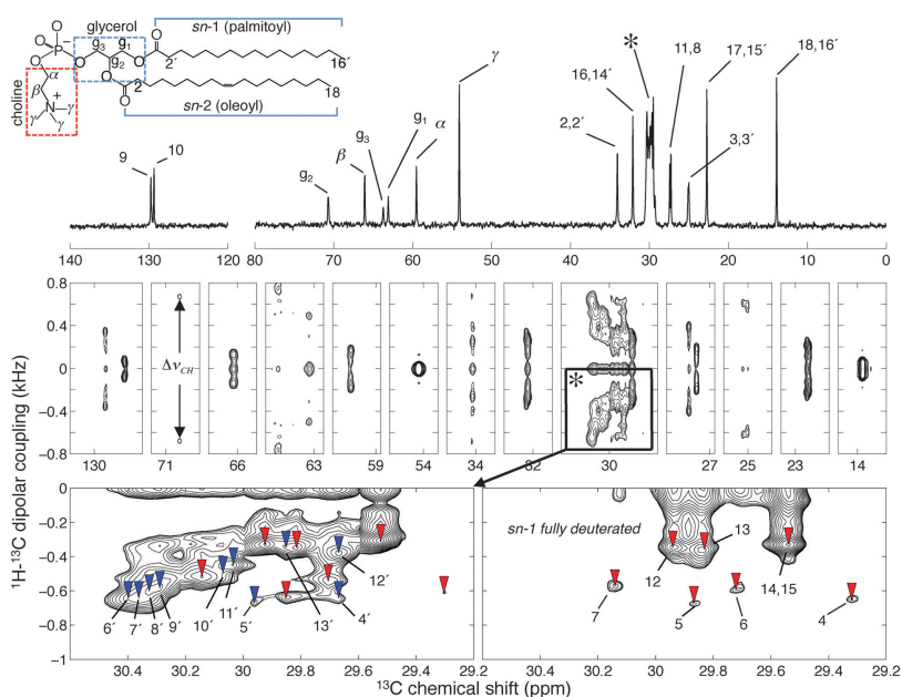
Fig. 2 2D ^1\text{H} - ^{13}\text{C} R-PDfL spectrum of fully hydrated POPC multi-lamellar vesicles recorded at 300 K and B_0 = 11.74 T with INEPT polarization transfer, 5 kHz magic-angle spinning, 50 kHz TPPM ^1\text{H} decoupling during ^{13}\text{C} acquisition, and 45 kHz R18 ^1\text{H} - ^{13}\text{C} dipolar recoupling in the indirect dimension. The peak for the \text{CH}_3 carbons \text{C}_{18} and \text{C}_{16}' is used as chemical shift reference at 13.9 ppm. Peak assignments as reported by Volke et al. 48 (*) Previously unassigned crowded spectral region around 30 ppm shown in detail for POPC (bottom, left) and POPC-d31 (bottom, right) multi-lamellar vesicles. Peaks from the sn -1 (palmitoyl) and sn -2 (oleoyl) chains are labeled with blue and red triangles respectively. The order parameters of the distinct carbons can be calculated from their splittings, \Delta\nu_{\text{CH}} .
