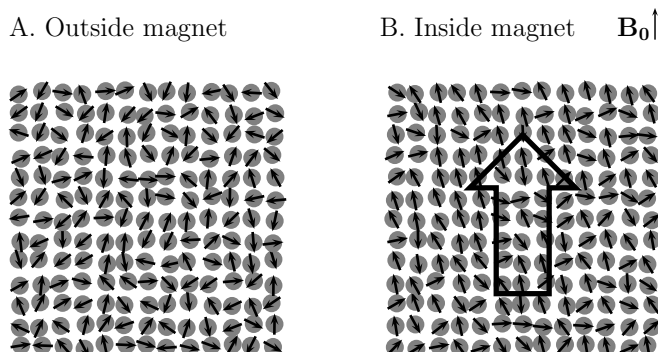
Figure 3.3: Net magnetization buildup by plunging a sample into a region with a strong magnetic field. On average, the magnetic moments become slightly aligned along the field. The magnetic field strengths currently used in NMR spectrometers are around 1 to 20 T. Comparatively to the Earth's magnetic field of around 25 to 65 \mu\text{T} , the magnetization buildup becomes 10^5 times higher. The orientation distribution used in (B) is overly exaggerated for the purpose of a clear illustration of the biased orientations of spin vectors \mu .
