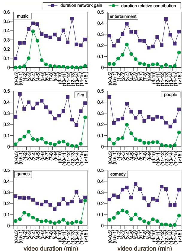
Fig. 5. Time distributed potential network caching gains of different video categories and their relative contributions to the total potential network gain.
