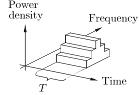
Fig. 3. Model of the distribution of energy in time and frequency from a packet transmission.
