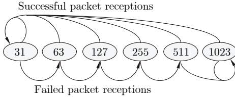
Fig. 9. Markov state diagram for the IEEE 802.11b contention window sizes.
