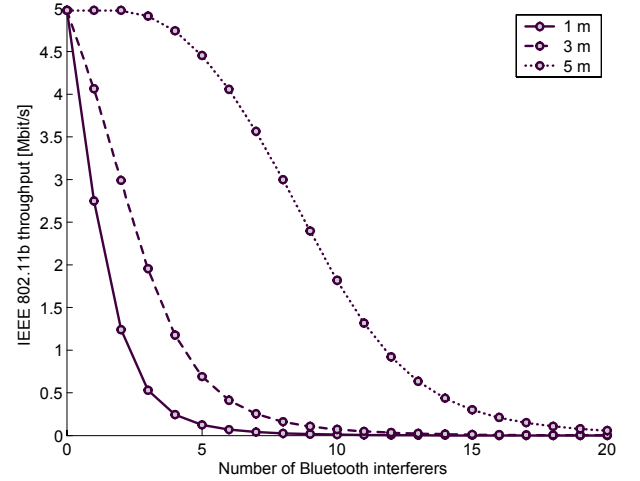
Fig. 10. IEEE 802.11b network throughput as functions of number of interfering Bluetooth networks for distances of 1, 3 and 5 meters to the interferers.
