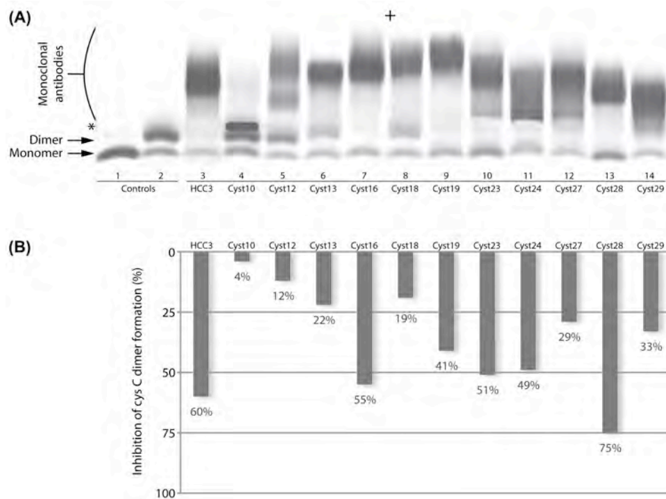
Figure 17. The capacity of 12 monoclonal antibodies to reduce dimerisation of cystatin C.
