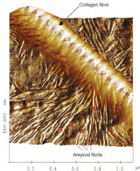
Figure 2. Tissue amyloid fibril deposition.
