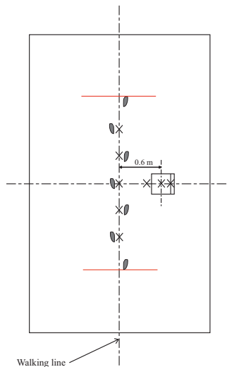
Figure 13: Measurement setup.
