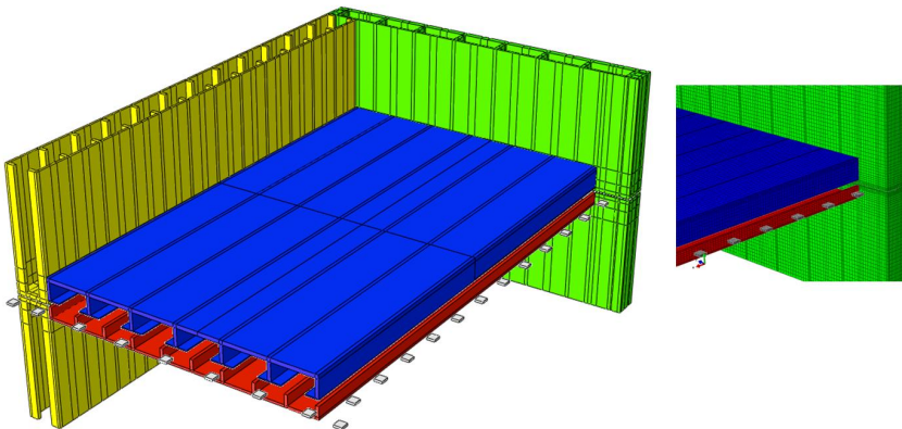
Fig. 6 - Case A with beams oriented lengthwise.
