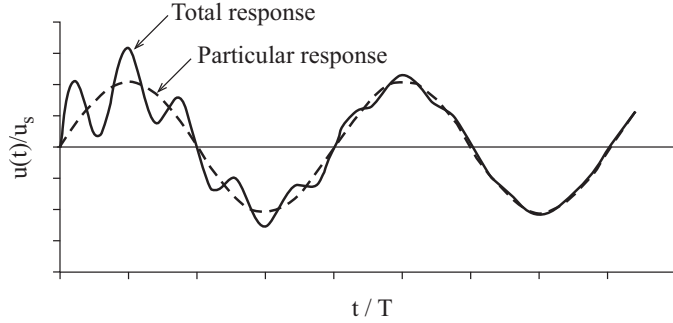
Figure 3.7: Example on the total response of a damped system subjected to a harmonic force, [54].
