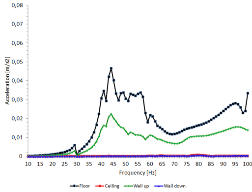
Fig. 8 - Case A widthwise. Acceleration magnitudes evaluated on the floor, ceiling, upper and bottom walls (left) and acceleration magnitudes evaluated on top and bottom of the Syldyn (right).
