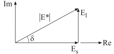
Figure 2: Complex representation of dynamic elastic modulus E^* .
