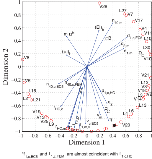
Figure 2: Vibration acceptability data – 2-D logistic PCA space. \circ : endpoints of the subject vectors; \bullet : endpoint of the average subject vector; — : objective parameter vectors.
