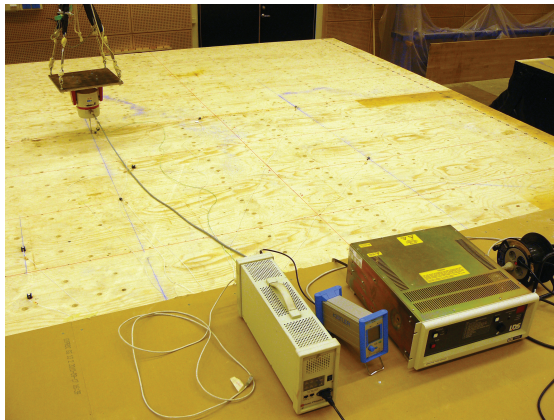
Figure 11: Shaker, accelerometers and other equipment used for the measurements.
