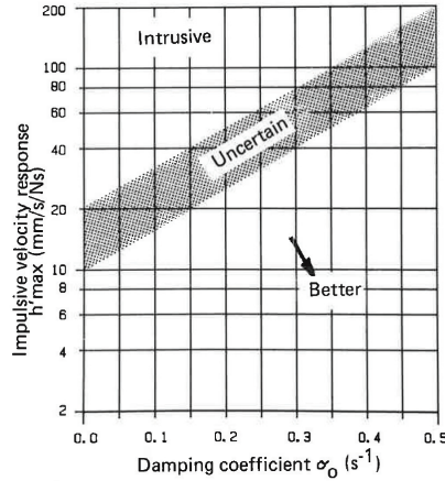
Figure 3.3: A preliminary proposal for classifying the response of a floor construction in terms of impact load [44].
