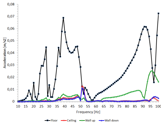
Fig. 9 - Case A lengthwise. Acceleration magnitudes evaluated on the floor, ceiling, upper and bottom walls (left) and acceleration magnitudes evaluated on top and bottom of the Syldyn (right).
