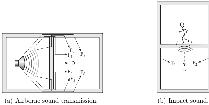
Figure 2.3: Sound transmission types. “D” denotes direct transmission whereas “ F_i ” indicates different flanking paths.
