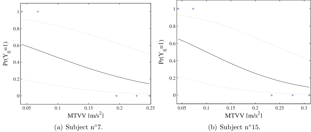
Figure 9: Vibration acceptability model involving MTVV – Individual regression lines for two subjects. —: median value; - -: lower and upper limits of the 95% credibility interval;+: actual binary responses.
