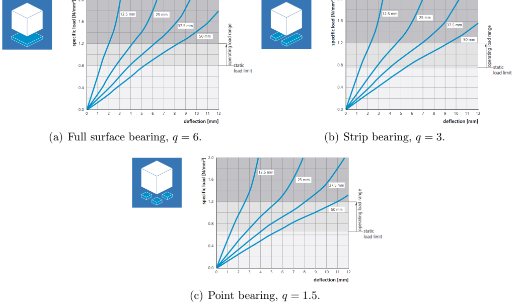
Figure 6: Quasi-static load deflection curve measured at a velocity of deformation of 1% of the thickness per second; testing between flat steel-plates; recording of the 3 rd loading; testing at room temperature [12].
