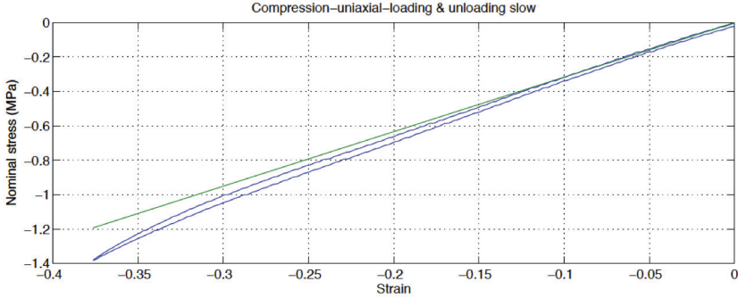
Figure 4: Compression-tests results. Loading and unloading curves (slow).
