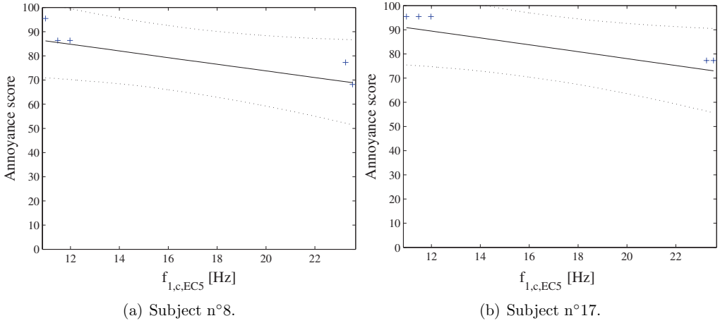
Figure 7: Vibration annoyance model involving f_{1,c,EC5} – Individual regression lines for two subjects. —: median value; - -: lower and upper limits of the 95% credibility interval; +: actual scores.
