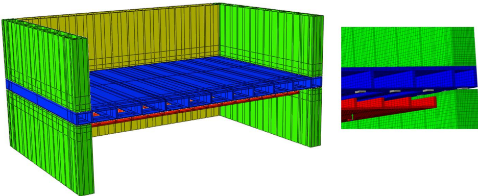
Fig. 7 - Case B with beams oriented widthwise.
