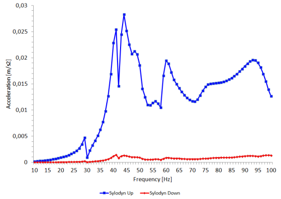
Fig. 8 - Case A widthwise. Acceleration magnitudes evaluated on the floor, ceiling, upper and bottom walls (left) and acceleration magnitudes evaluated on top and bottom of the Syldyn (right).
