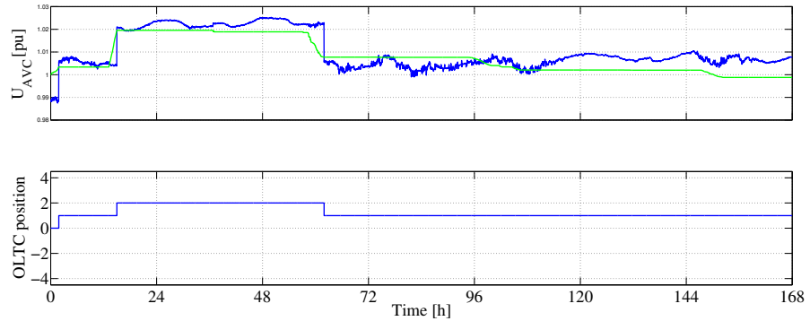
Figure 4.11: Voltage setpoint for the AVC relay (green line in upper subfigure) and actual voltage at the medium voltage busbar of the HV/MV substation (blue line in upper subfigure) and the current tap changer position of the OLTC at the HV/MV substation (lower subfigure).
