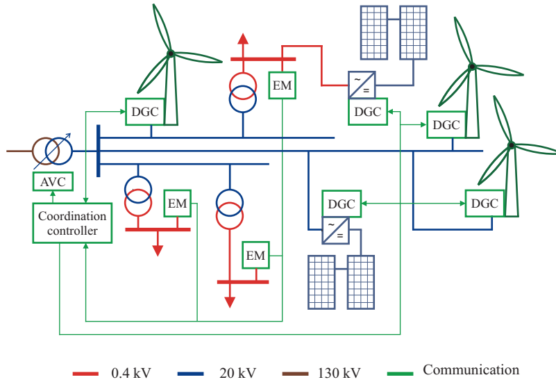
Figure 3.1: Scheme over coordinated voltage control in a distribution system with three typical feeder types and DG at low and medium voltage level.
