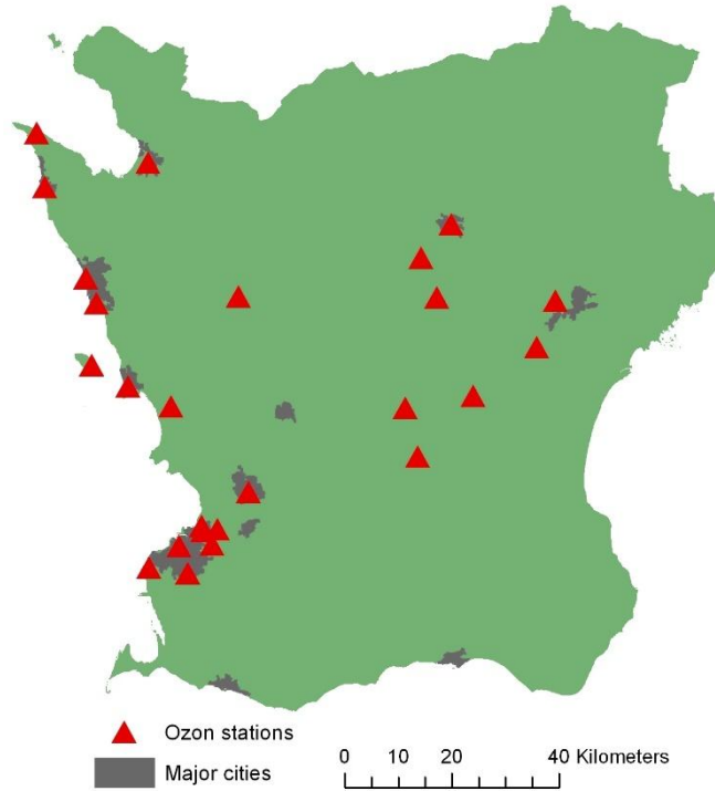
Figure 4 Ozone monitoring stations used in Paper IV.
