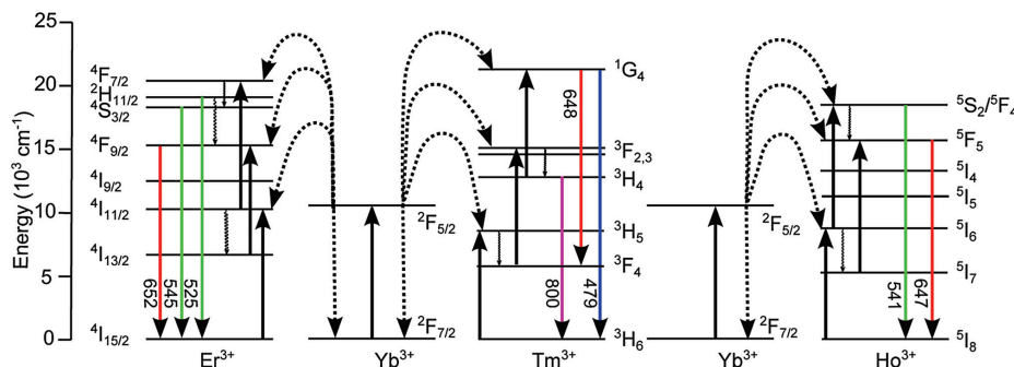
Figure 1 (online color at: www.lpr-journal.org ) Energy level structure and proposed UC mechanisms of the \text{Yb}^{3+} , \text{Er}^{3+} / \text{Tm}^{3+} / \text{Ho}^{3+} co-doped UCNP under excitation at 975 nm.
