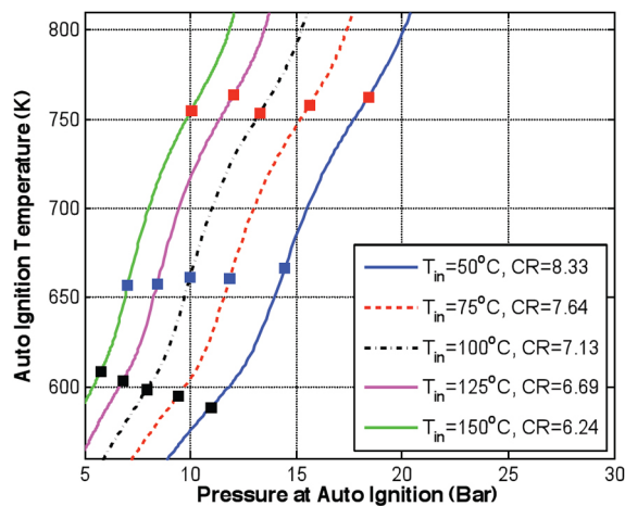
Figure 15. Auto ignition pressures and temperatures for PRF 20.
