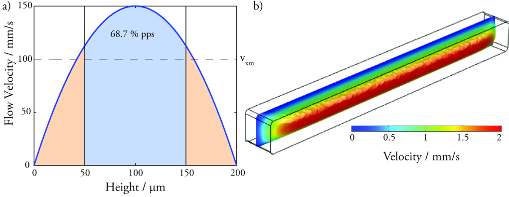
Figure 9: The parabolic flow profile between two plates with 200 \mu\text{m} spacing (a), and a simulation of the flow in a trapping capillary (b), which is 200 \mu\text{m} high and 2 mm wide. As seen, the plate approximation accurately describes the central parts of the channel but needs adjustment close to the wall.
