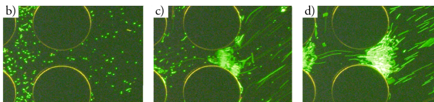
Figure 3: In insulator-based dielectrophoretic trapping a non-uniform electric field is created by the insulator posts. The normalized intensity in the simulation (a) shows how the field gradient allows Escherichia coli captured in the sequentially taken photos (b-d) Adapted with permission from (B. H. Lapizco-Encinas, et al., Anal Chem 76 (6), 1571-1579 (2004)). Copyright (2004) American Chemical Society.
