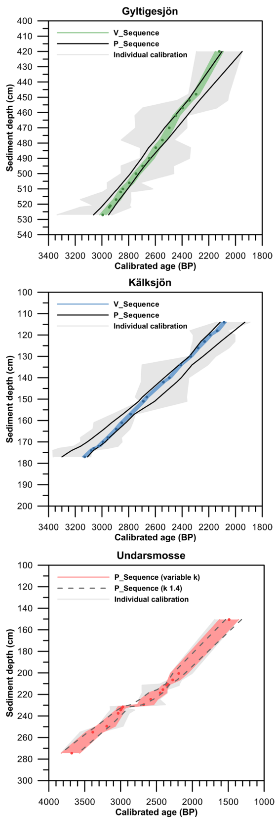
Figure 4. Comparison between different age-depth models of Gyltigesjön, Kälksjön and Undarsmossen. The final age models used in Papers I-IV are indicated by green/blue/pink shading. Mean ages for the final age models are indicated by filled circles.
