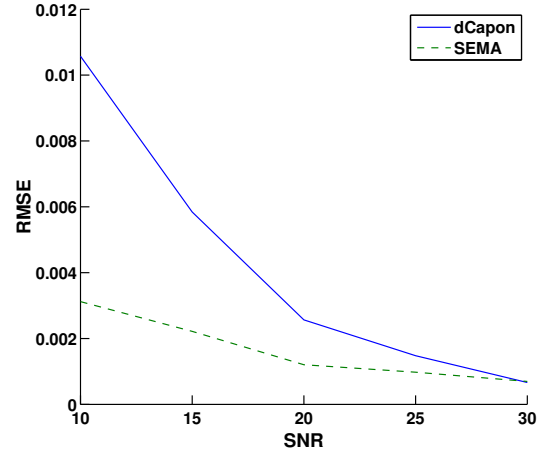
Fig. 2. The RMSE of the damping estimation as a function of SNR. The signal contains three modes.
