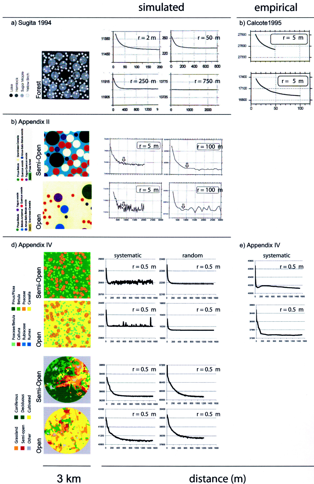
Figure 13. Summary of the simulated and empirical estimates of relevant source area of pollen (RSAP) of basins of various size. In the first column: the vegetation maps of the simulated landscapes, in the second and third the simulated and in the fourth column the empirical estimates of RSAP derived from the likelihood function scores. The radius ( r ) of the basin is indicated in each figure. a) simulations of four different basin size in forested vegetation in northern Michigan, USA (Sugita, 1994), b) empirical estimates of RSAP for forest hollows northern Michigan, USA (upper) and north west Wisconsin, USA (lower) (Calcote, 1995). c) simulation of hollows and small lakes in Open and Semi-Open Region of southern Sweden (Appendix II), d) simulated and e) empirical estimates of RSAP for moss polsters sites Open and Semi-Open Region of southern Sweden (Appendix IV). See also Table 1.
