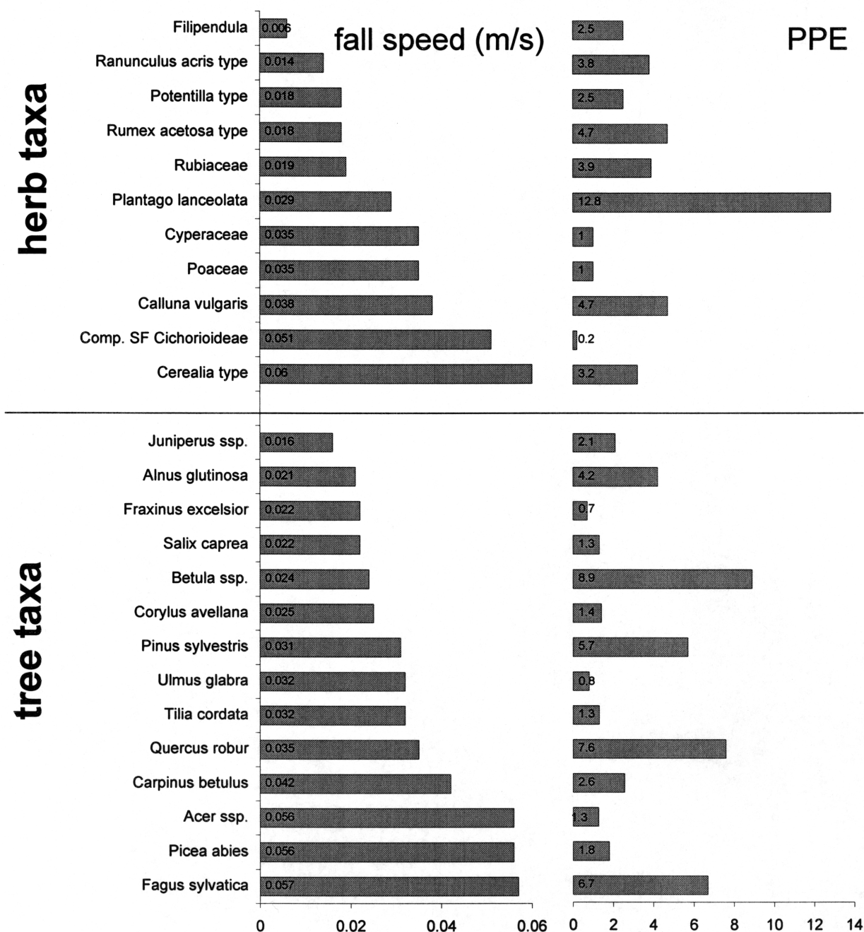
Figure 12. The fall speed (m/s) and pollen productivity for 25 plant taxa characteristic of the cultural landscape of southern Sweden. The pollen productivity estimates are relative to Poaceae set to one (see further details in Appendices II and III).
