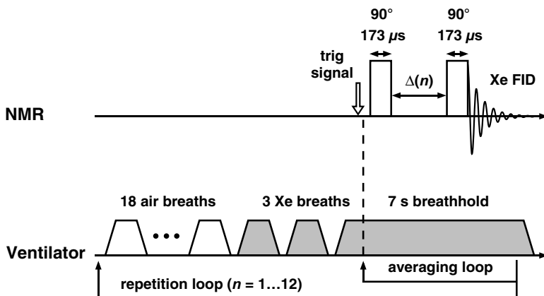
Figure 5. Schematics of the ventilator operation and NMR data acquisition. A repetition cycle consisted of 18 air breaths followed by 3 xenon breaths. After the last xenon inspiration, a 90^\circ RF pulse was applied to destroy the signal in tissue and blood, followed by a second 90^\circ RF pulse generating a FID from the xenon in tissue and blood. The interpulse delay \Delta(n) was increased between successive repetitions.
