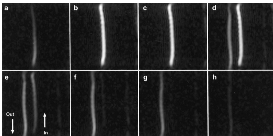
Fig. 2. a–h) EPI images showing a time series of flowing \text{Hp } ^{129}\text{Xe} , acquired at 1.5-s intervals. The acquisition time of each image was 44 ms. The flow direction is indicated in (e). The mean flow velocity was 15 cm/s and the \text{HpXe} polarization level was estimated to 2%.
