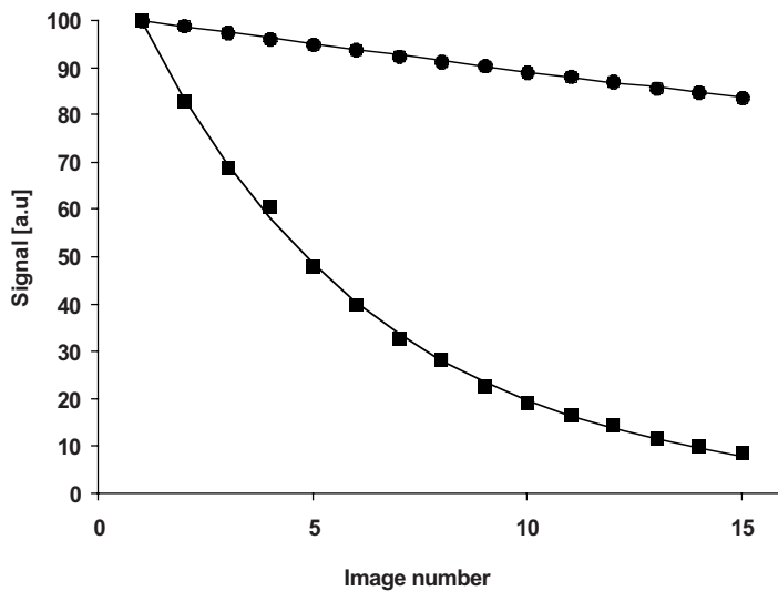
Figure 3. Signal variation in 15 consecutively acquired images using the flip-back technique and \theta = 180^\circ for HP ^{13}\text{C} in water (circles) and in vivo (squares). Signal is preserved from one image to the next, but decays faster in vivo than in the water. Assuming that no magnetization is lost in the flip-back process or between image acquisitions, the signal drop reflects the T_2 relaxation. The lines in the figure are mono-exponential fits to the measured values, yielding T_2 \approx 18 s for the ^{13}\text{C} molecule in water, and T_2 \approx 1.3 s in vivo .
