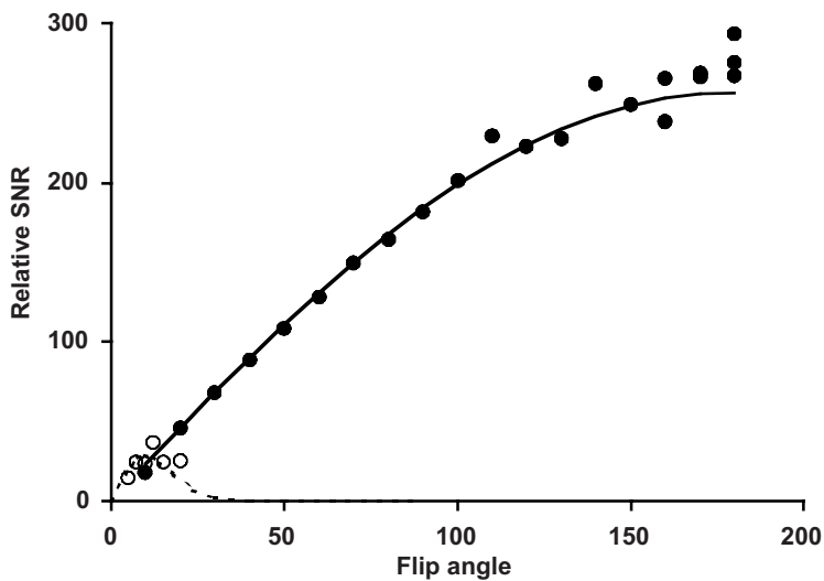
Figure 4. Flip angle dependence for the trueFISP pulse sequence and the hyperpolarized ^{13}\text{C} -based contrast medium. Measured values (●) and theoretical values calculated using Eq. [4] (solid line) agree very well. The optimal flip angle is 180°. The two data sets are normalized at 70°. For comparison, the corresponding calculated (dashed line) and measured values (○) for a FLASH pulse sequence are also plotted.
