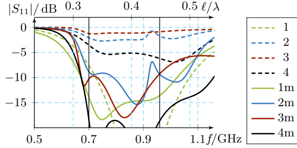
Figure 20: 1, 2, 3, 4—magnitudes of the S_{11} parameter at the input of the corresponding structures depicted in Fig. 19. 1m, 2m, 3m, 4m—magnitudes of the S_{11} parameter at the input of the matching networks of Fig. 19 terminated with the corresponding structures depicted on the first row in Fig. 19.
