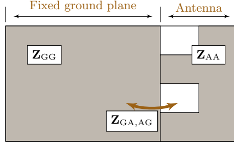
Figure 3: Schematic illustration of antenna embedded in a wireless terminal. Gray shading—metallic parts.
