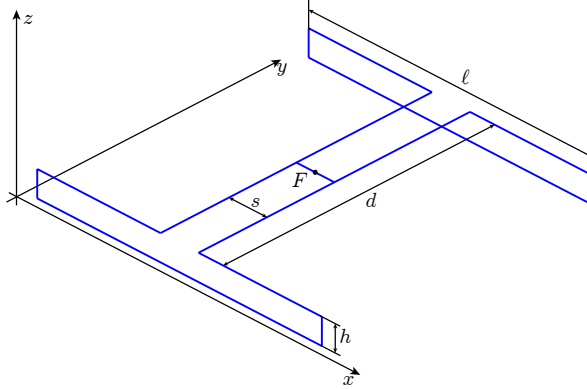
Figure 8: Two element array of folded dipoles with \ell = 492.9 mm and d = 470 mm.
