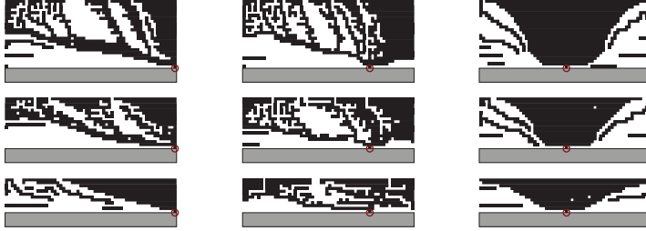
Figure 2: Example of antenna regions of structures optimized for multiband minimum Q . Rectangular regions 130 \times 65 \text{ mm}^2 with fixed rectangular ground planes and antenna regions extending 20% (top row), 15% (middle row), and 10% (bottom row) of the entire structure area as depicted in Fig. 1. Fixed feeding edges are circled. Part of the ground plane is shaded.
