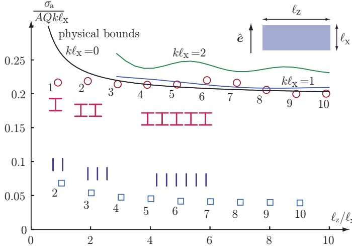
Figure 10: Illustrations of the physical bounds on the effective antenna aperture, \sigma_a , of planar rectangular circumscribing regions with height \ell_x , width \ell_z , and physical area A = \ell_x \ell_z .
