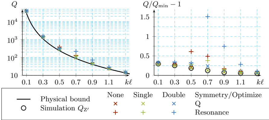
Figure 9: Left—GA-optimized antenna Q -factors compared with the physical bound [37, 38] for rectangular regions. The smallest Q -factor obtained in 5 GA runs for each symmetry (none, single—along \ell , and double—along \ell and w ) and optimization criterion ( Q -factor or resonance) is depicted. Right—deviation of the Q -factors depicted to the left relative to the physical bound Q_{\min} [37, 38]. The deviations of the Q -factors (5.13) evaluated from the input impedance computed by ESI-CEM [24] are included for the antennas having the smallest Q -factor for each frequency, regardless of optimization criterion or symmetry.
