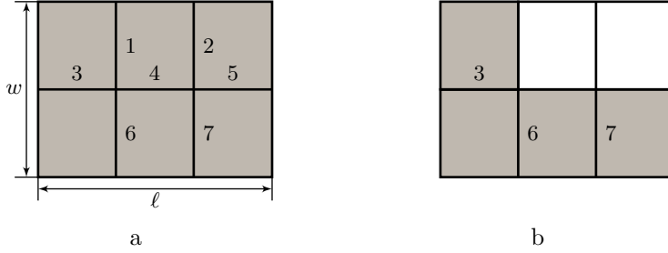
Figure 7: Illustration of a mother structure (a) and an individual derived from it (b). Gray-shaded rectangles—PEC mesh elements. Basis functions are numbered.
