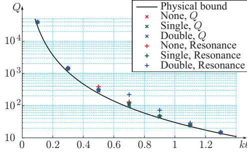
Figure 3: Optimized antenna Q -factors compared with the physical bound [6, 9, 10] for rectangular regions. The best result from 5 runs for each symmetry (none, single and double) and optimization criterion ( Q -factor or resonance) is depicted.
