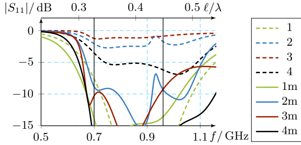
Figure 5: Magnitude of S_{11} at the input of the structures depicted in Fig. 4 without matching network, the curves labeled 1, 2, 3 and 4, and with the matching networks sketched in Fig. 6, the curves labeled 1m, 2m, 3m and 4m.
