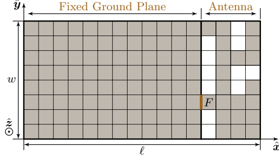
Figure 1: Example of discretized radiating structure with a fixed rectangular ground plane. Gray shaded elements represent metallic patches. The feeding edge is marked F .
