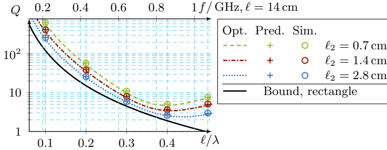
Figure 17: Q -factors of antennas optimized using a GA, “Pred.”, compared to corresponding Q -factors (4.28) of D/Q -optimum current densities, “Opt.”, for the bent-end model illustrated in Fig. 8c with \ell_2 = 0.7 cm, 1.4 cm and 2.8 cm and \ell = 14 cm. The input impedance of the GA-optimized structures, computed by ESI-CEM [24], has been used to calculate the Q -factors “Sim.”. The physical bound on Q for a rectangular, infinitely thin, 14 \times 7 cm 2 , PEC sheet is depicted in solid black line [37, 38].
