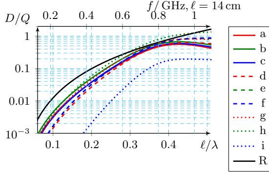
Figure 8: Physical bounds on D/Q for the structures depicted in Fig. 7 obtained using the convex optimization formulation (2.24), [10], when only the antenna region (black in Fig. 7) is optimized. The physical bound on D/Q for a rectangular PEC surface 14 \times 7 \text{ cm}^2 , [11], is depicted in solid black line and labeled “R.”
