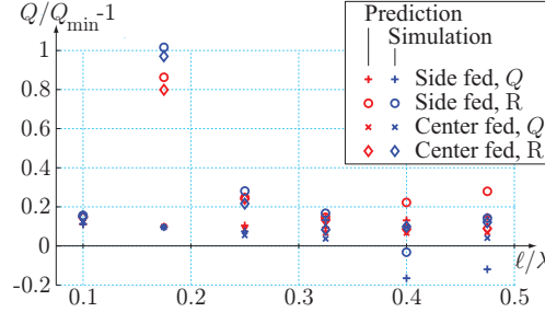
Figure 7: Deviation of optimized antenna Q -factors relative to the physical bound [8] for 15 % antenna regions (see Fig. 2). The smallest Q -factor from five optimization algorithm runs is labeled “Prediction”. The Q -factors computed using the results in [7, 25, 26] from simulation data for the smallest Q antennas are labeled “Simulation”. Side and center feeding has been considered for structures optimized for Q -factor and resonance (R).
