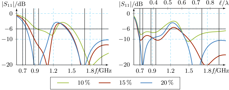
Figure 16: Left—magnitude of the reflection coefficient at the input of the structures with antenna regions depicted in Fig. 15, third row from the top. Right—magnitude of the reflection coefficient at the input of the matching networks of Fig. 15 terminated with the corresponding half-way-fed structures of Fig. 15. The curves correspond to antenna regions extending 10%, 15% and 20% at one end of the structure length as in Fig. 8b.
