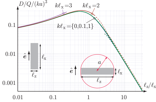
Figure 3: Bound on D/Q for a planar rectangle with sides \ell_x and \ell_z for k\ell_x = \{0, 0.1, 1, 2, 3\} and \hat{\mathbf{k}} = \hat{\mathbf{y}} normal to the rectangle and \hat{\mathbf{e}} = \hat{\mathbf{x}} . The solid curves show the bounds determined for irrotational surface currents, \nabla_t \times \mathbf{J} = \mathbf{0} , using (4.10). The dashed curves show the corresponding asymptotic results in [10].
