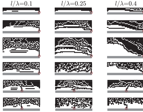
Figure 8: Example of antenna regions of structures simulated in Efield. Shaded – part of the ground plane. First three rows from top to bottom: side fed antenna regions occupying 6 %, 15 %, 25 % of antenna length optimized for Q -factor. Row 4: side fed 15 % antenna regions optimized for resonance. Rows 5 and 6: center fed 15 % antenna regions optimized for Q -factor and resonance, respectively. Feeding edges are circled.
