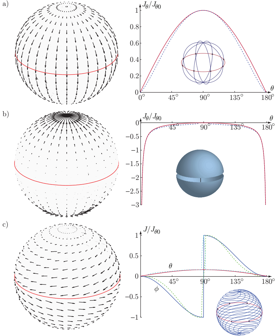
Figure 5: Examples of surface current distributions on spheres with the surface charge density \rho = \rho_0 \cos \theta . a) folded spherical dipole with \mathbf{J} \approx J_{\theta 0} \hat{\theta} \sin \theta . b) capped spherical dipole with \mathbf{J} \approx J_{\theta 0} \hat{\theta} (\sin \theta - 1/\sin \theta) . c) folded spherical helix with \mathbf{J} \approx J_{\theta 0} (0.15 \hat{\theta} \sin \theta - \hat{\phi} \text{sign}(\cos \theta) \sin^2 \theta) .
