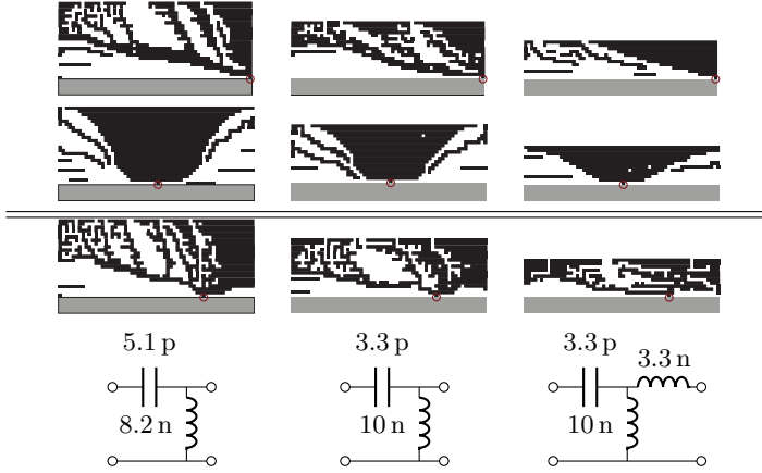
Figure 15: Antenna regions, black, of structures optimized for simultaneous multiband minimum Q . Circled—fed mesh edges on the borderline between antenna region and ground plane, at the side of the model in the w -direction (first row from the top), in the center (second row), and half way between center and side (third row). Bottom row—matching networks for the structures on the third row from the top, in SI units. Gray shaded—part of the ground plane. From left to right columns correspond to antenna regions extending 20 %, 15 %, and 10 % of the entire device model, at one end in the \ell -direction, as depicted in Fig. 8b.
