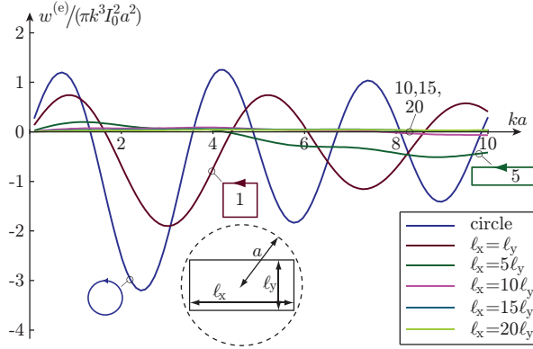
Figure 11: Stored electric energy for circular (A.1) and rectangular loop currents.
