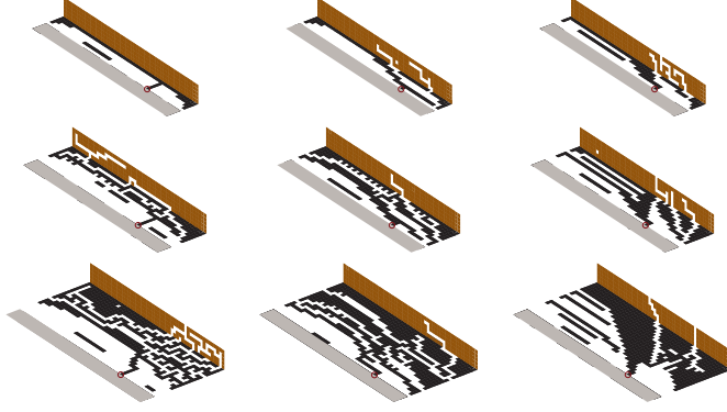
Figure 18: Example of genetic algorithm optimized structures (gray shading—part of the ground plane, black—antenna region part coplanar with the ground plane, bronze—antenna region part normal to the ground plane) with Q -factors depicted in Fig. 17 for \ell/\lambda = 0.1 (left column), 0.3 (middle column) and 0.5 (right column), and \ell_2 = 0.7 cm (top row), 1.4 cm (middle row), and 2.8 cm (bottom row). Feeding edges are circled.
