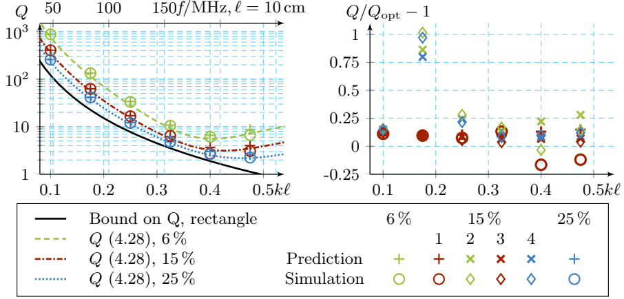
Figure 11: GA-optimized antenna Q -factors, labeled “Prediction”, compared with Q -factors (4.28), denoted Q_{\text{opt}} to the right, of D/Q -optimum current distributions (see Sec. 4.3.1). The physical bound on Q for a rectangular, infinitely thin, PEC sheet [37, 38] is included for illustration. The Q_Z -factors (5.13) of the structures having the Q -factors “Prediction” are labeled “Simulation” because the former are computed from ESI-CEM [24] simulation data. Antenna regions extend 6%, 15% and 25% of the model area, as in Fig. 8b. The cases 6%, 15%–1 and 25% are structures optimized for minimum Q , fed at the side of the rectangular model in the w -direction. The case 15%–2 represents structures optimized for resonance fed, at the side. The cases 15%–3 and 15%–4 are structures fed at the center of the rectangular model in the w -direction, optimized for minimum Q and resonance, respectively.
