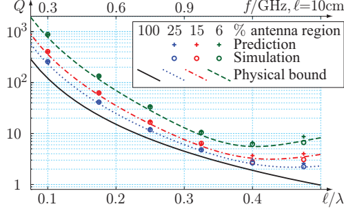
Figure 6: Optimized antenna Q -factors compared with the physical bound. The smallest Q -factor of five optimization algorithm runs per frequency and antenna region size is labeled “Prediction”. The Q -factors computed using the results in [7, 25, 26] from simulation data for the smallest Q antennas are labeled “Simulation”. The physical bounds for radiating structures with rectangular ground planes [8] and antenna regions occupying 6, 15 and 25 % of antenna length (see Fig. 2) are depicted in dashed, dash-dot and dotted line, respectively. The physical bound for antennas limited to rectangular regions [6, 9, 10] is depicted in solid line.
