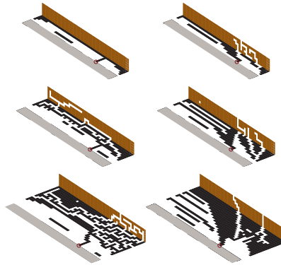
Figure 3: Example of genetic algorithm optimized structures (gray shading—part of the ground plane, black—antenna region part coplanar with the ground plane, bronze—antenna region part normal to the ground plane) with Q -factors depicted in Fig. 2 for \ell/\lambda = 0.1 (left column) and \ell/\lambda = 0.5 (right column), and \ell_2 = 0.7 cm (top row), 1.4 cm (middle row), and 2.8 cm (bottom row). Feeding edges are circled.
