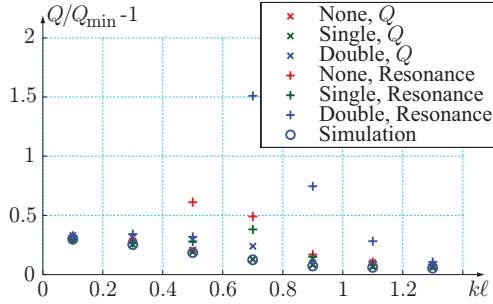
Figure 4: Deviation of the Q -factors depicted in Fig. 3 relative to the physical bound Q_{\min} [6, 9, 10]. The deviations of the Q -factors computed from simulation data using the procedure in [7, 26] are also included.
