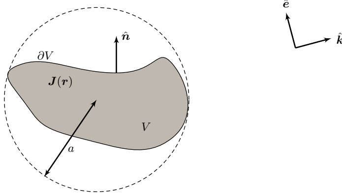
Figure 1: Illustration of radiating structure occupying a volume V which has the bounding surface \partial V with the outward pointing normal vector \hat{n} . The smallest sphere that can enclose the antenna, i.e. , the smallest circumscribing sphere, has the radius a . The wave and polarization vectors, \hat{k} and \hat{e} , respectively, are sketched for the far field region.
