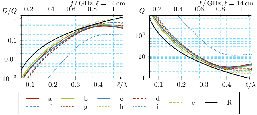
Figure 22: Left—physical bounds on D/Q for the structures depicted in Fig. 21 obtained using the convex optimization formulation (4.26) when only the antenna region (black in Fig. 21) is optimized. Right— Q -factors (4.28) of the D/Q -optimum current densities giving the curves to the left. The physical bounds on D/Q and Q for a rectangular PEC surface 14 \times 7 \text{ cm}^2 , [37–39], is depicted in solid black line and labeled “R”.
