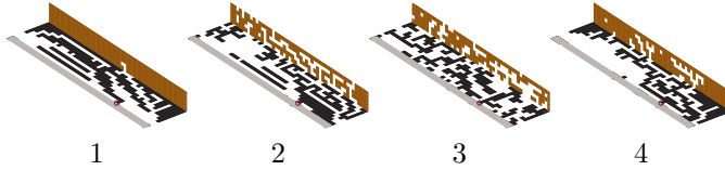
Figure 4: GA-optimized structures whose Q -factors are listed in Table 1. Gray shading—part of the ground plane, black—antenna region part coplanar with the ground plane, bronze—antenna region part normal to the ground plane. Feeding edges are circled.
