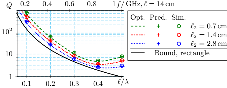
Figure 2: The Q -factors of antennas optimized using a genetic algorithm (“+”) compared to corresponding Q -factors of D/Q -optimum current densities, [10], for the bent-end model illustrated in Fig. 1 with \ell_2 = 0.7 cm, 1.4 cm and 2.8 cm and \ell = 14 cm. The input impedance of the GA-optimized structures, computed by ESI-CEM, [7], has been used to calculate the Q -factors “o” using a resonance model [9, 27, 28]. The physical bound on Q for a rectangular PEC surface 14 \times 7 cm 2 , [11], is depicted in solid black line.
