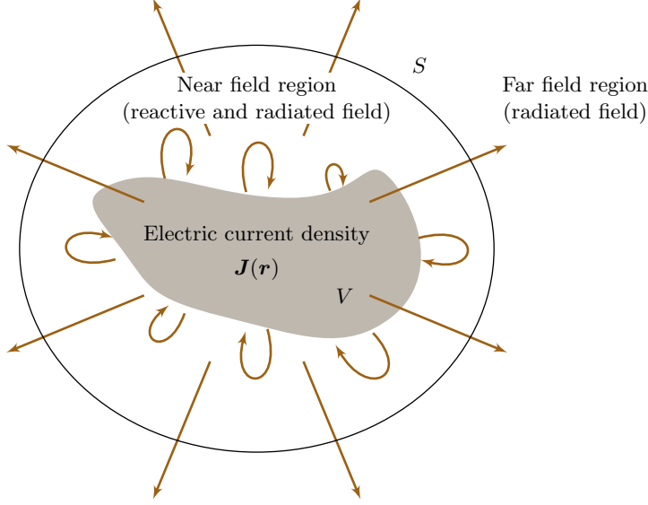
Figure 2: Radiating structure occupying the volume V where the current density \mathbf{J}(\mathbf{r}) is excited. The arrows illustrate, in a simplified manner, the power flow in the near and far field regions of the structure.
