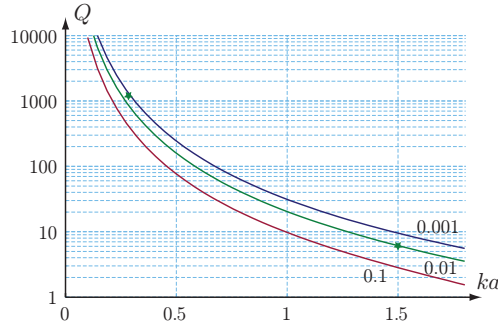
Figure 8: Q factor for the optimal current distributions corresponding to the D/Q bound in Fig. 7. The numerical results for strip dipoles with \xi = 0.01 and ka \approx \{0.28, 1.49\} are indicated by the stars.
