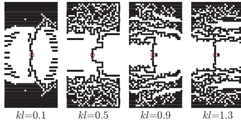
Figure 5: Four of the structures simulated in Efield whose Q -factors are depicted in Fig. 3. Feeding edges are circled.
