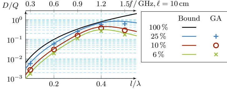
Figure 13: GA-optimized antenna D/Q -ratios (4.22), marks, compared with physical bounds on D/Q (4.24) for a rectangular wireless device model in which the antenna may occupy 6%, 10% and 25% of the device at one end, see Fig. 8. The physical bound on the D/Q -ratio of a rectangular, infinitely-thin, PEC sheet [37–39] is labeled “100 %”.
