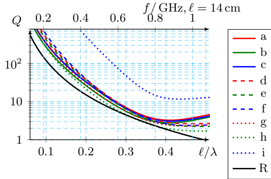
Figure 9: The Q -factors (2.6) achieved by the currents that give the optimum D/Q -values depicted in Fig. 8. The Q -factor of a 14 \times 7 \text{ cm}^2 PEC rectangle, [11], is labeled “R.”
