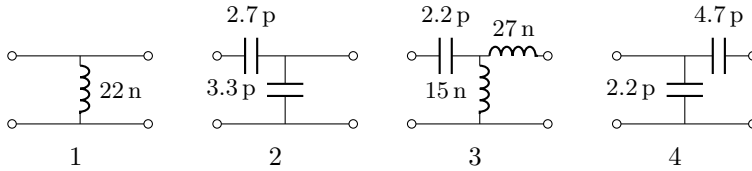
Figure 6: Matching networks designed for the structures depicted in Fig. 4 to yield less than -6 dB reflection coefficient magnitude between 700 \dots 960 MHz (solid curves in Fig. 5). Component values in SI units. Matching networks numbered as structures in Fig. 4—left to right and top to bottom.
