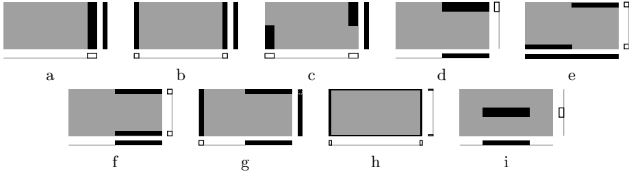
Figure 7: Nine simplified wireless-device models limited to a parallelepiped, consisting of a planar ground region extending 90 % of one length \times width face, and an antenna region occupying 10 % of the parallelepiped volume. Three side views are depicted for a-g and i, i.e. , structures as seen along the length, width and height. A side view along the height and two sections at the symmetry planes are depicted for h. Gray shading—ground plane; black—antenna region, [5, 6].
