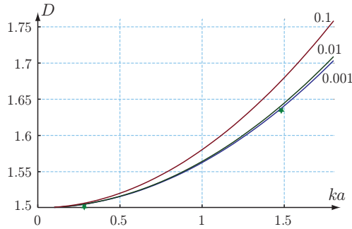
Figure 9: Directivity for the optimal current distributions corresponding to the D/Q bound in Fig. 7. The numerical results for strip dipoles with \xi = 0.01 and ka \approx \{0.28, 1.49\} are indicated by the stars.
