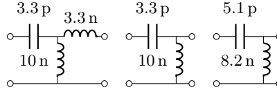
Figure 4: Matching networks for the structures with antenna regions depicted in Fig. 2 middle column, in SI units. From left to right the networks correspond to antenna regions extending 10%, 15% and respectively 20%.
