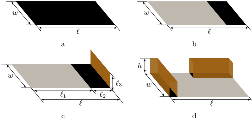
Figure 8: Four antenna design situations, labeled a–d, analyzed in Secs 6.1–6.4, respectively. Gray shading—fixed regions, i.e. , ground plane. Black and bronze—regions where structures can be optimized, i.e. , antenna region [17].
