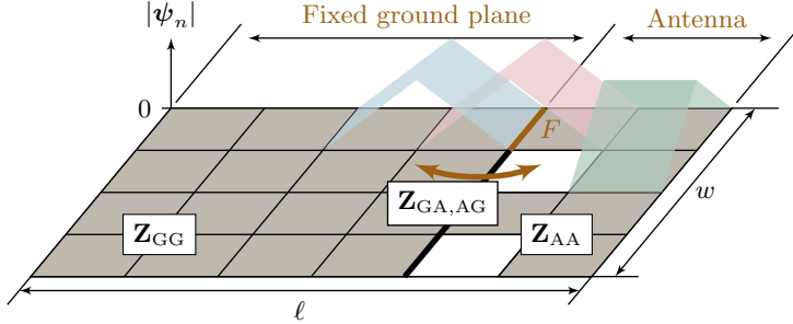
Figure 4: Illustration of discretization for a structure using rectangular mesh elements. Metal areas are depicted in gray shading. The amplitudes of three of the total 6 \times 3 + 5 \times 4 - 4 - 3 basis functions are depicted in blue, pink and green shading. The feeding edge is marked F . The locations of basis and testing functions when a block matrix decomposition is applied to the impedance matrix, \mathbf{Z} , are illustrated by the positions of the resulting blocks, \mathbf{Z}_{AA} , \mathbf{Z}_{GG} , \mathbf{Z}_{GA} and \mathbf{Z}_{AG} , where the subscripts G and A denote the ground plane and antenna region, respectively.
