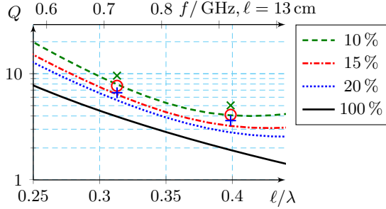
Figure 3: The Q -factors (2.6) of the structures with antenna regions depicted in Fig. 2 middle column (top row “+”, middle row “o”, and bottom row “x”) compared to the physical bounds [7, 9] for rectangular structures with antenna regions 20 %, 15 %, and respectively 10 % of the entire structure as in Fig. 1. The physical bound for structures limited to entire rectangular regions [8] is depicted in solid line (100 %). The frequency scale for an \ell = 13 cm structure is included.
