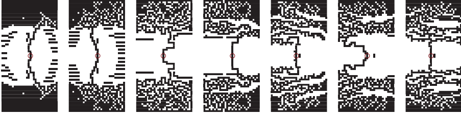
Figure 10: The structures simulated in ESI-CEM, [24], whose Q -factors are the smallest per kl -value in Fig. 9. The Q_{Z'} -factors (5.13) of these structures are depicted with circular marks in Fig. 9. Feeding edges are circled. From left to right— kl = 0.1, 0.3, 0.5, 0.7, 0.9, 1.1, 1.3 .
