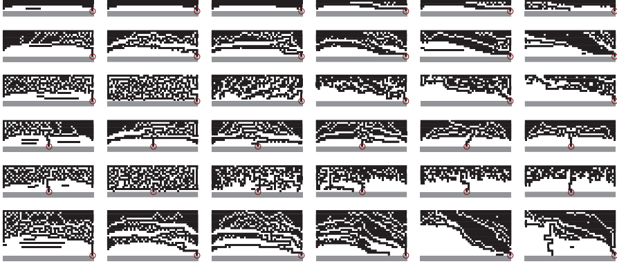
Figure 12: Antenna regions of the structures whose Q -factors are depicted in Fig. 11. Each structure has a Q -factor labeled “Prediction” and a Q_{Z'} -factor labeled “Simulation” in Fig. 11. Shaded—part of the ground plane. Feeding edges are circled. The rows from top to bottom correspond to the columns 6 %, 15 %–1, 15 %–2, 15 %–3, 15 %–4 and 25 % in the legend of Fig. 11.
