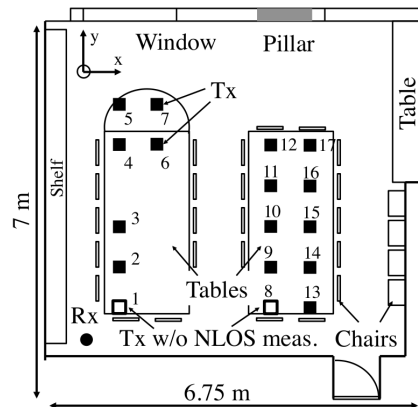
Figure 3: Floor plan of the 60 GHz MIMO radio channel measurements.
