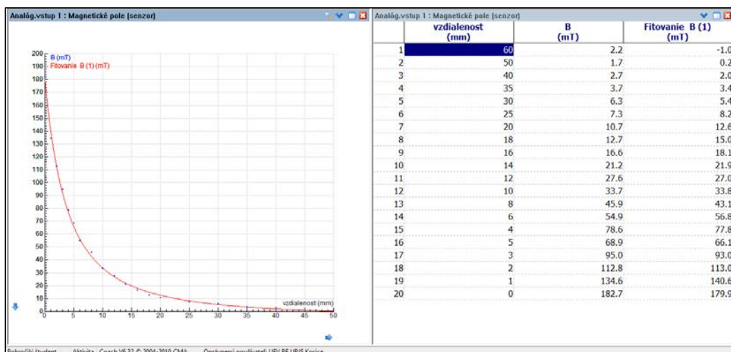
Figure 3. Dependence of the intensity of magnetic induction on the distance measured by the magnetic sensor in front of the magnet
