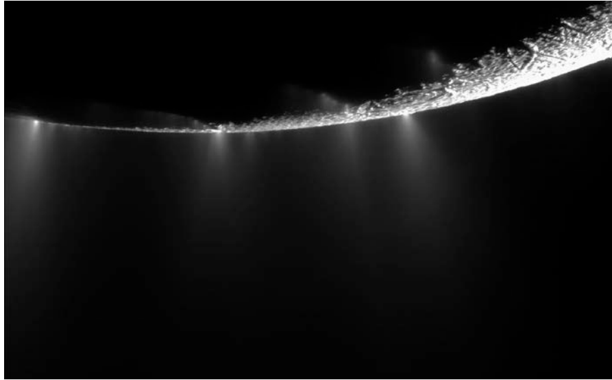
Figure 5. Cryovolcanic activity on Saturn's satellite Enceladus (near its south pole). In the picture we can see more than 30 individual jets of icy particles. On the surface there are the “tiger stripes” – the fissures that spray icy particles, water vapour and organic compounds.
