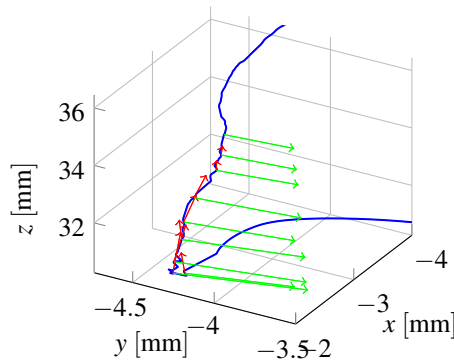
Figure 2.17 Peg-in-hole operation zoomed in. The trajectory is in blue. The red arrows are proportional to the contact forces and green arrows to the torques (the right-hand convention).
