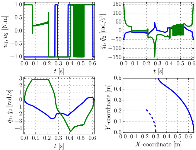
Figure 4.5 Solution of (4.16). The blue and green curves correspond to joint one and two, respectively. In the X-Y plot, the solid and the dashed line correspond to the position of the end-effector and the second joint, respectively.
