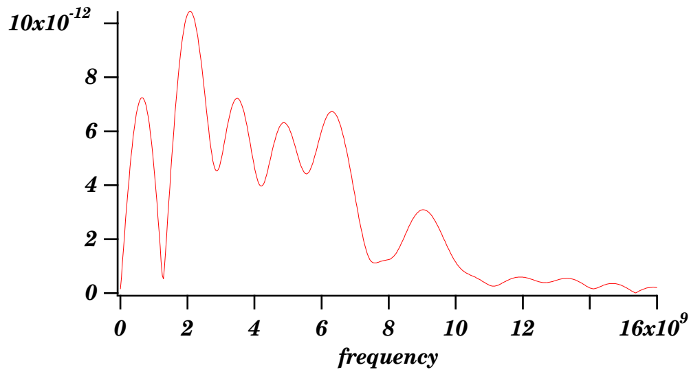
Figure 11 d: The DFT of the reflected waveform.
