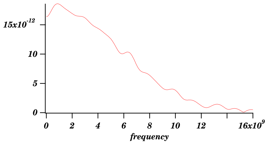
Figure 11 c: The DFT of the incident waveform.
