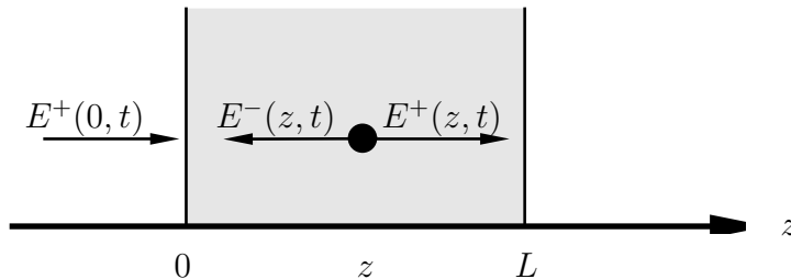
Figure 5: Wave splitting.
