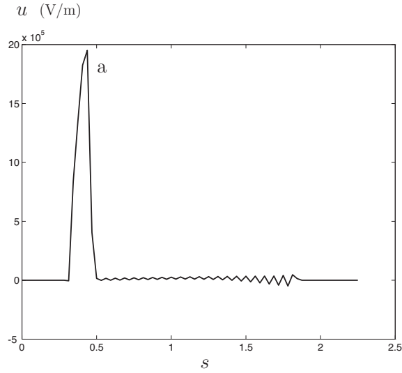
Figure 20: Time evolution of the pulse in Figure 18 ( x = 20/64 ).
