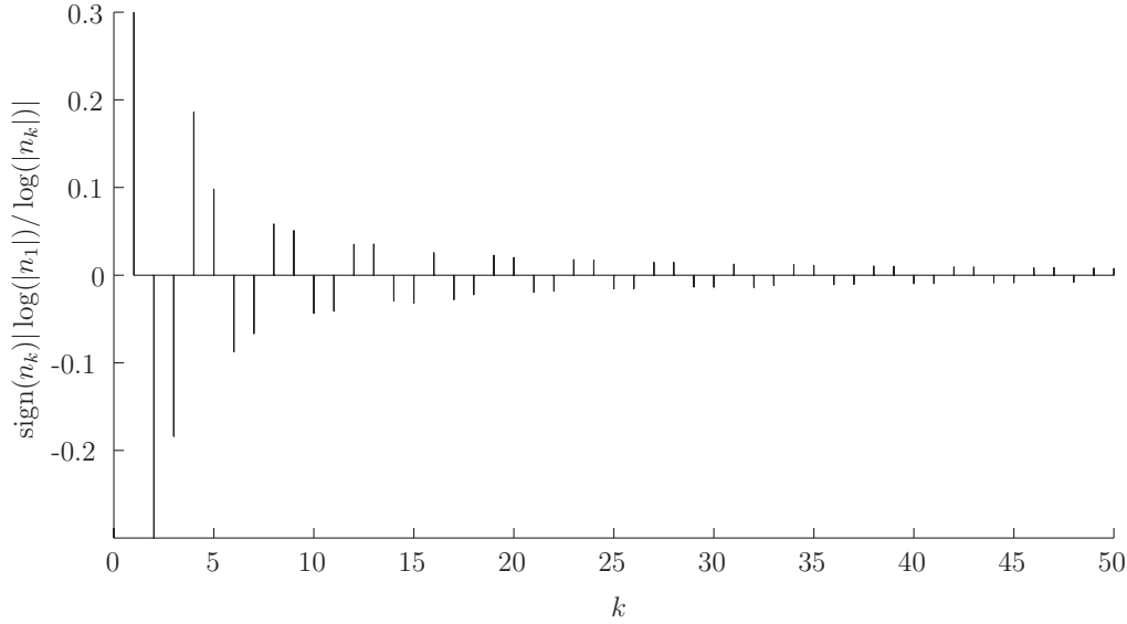
Figure 5: The sign of the coefficients n_k for a double-resonance Lorentz medium with \omega_{p1} = \sqrt{5} \times 10^{16} rad/s, \omega_{01} = 10^{16} \times rad/s, \nu_1 = 0.2 \times 10^{16} \text{ s}^{-1} and \omega_{p2} = \sqrt{20} \times 10^{16} rad/s, \omega_{02} = 10 \times 10^{16} rad/s, \nu_2 = 0.56 \times 10^{16} \text{ s}^{-1} . The signature +- -+ is violated at k = 17 . This means that the expansion (6.8) has to be truncated at k < 17 . The coefficients \chi_k have the same signs as n_k for the k in this figure. The corresponding propagator is depicted in Figure 6.
