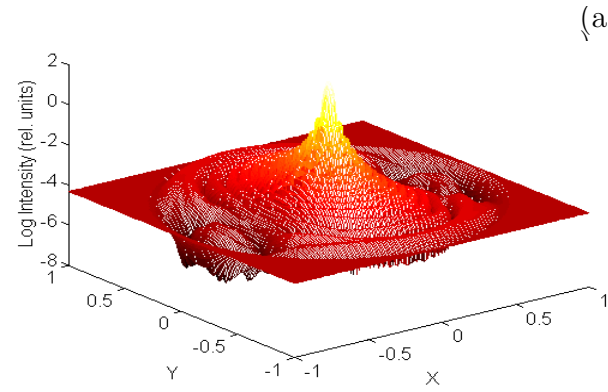
Volume equivalent of a RBC, Prolate II, incident angle=90°
