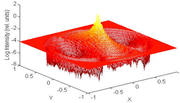
Volume equivalent of a RBC, Prolate III, incident angle=90°
