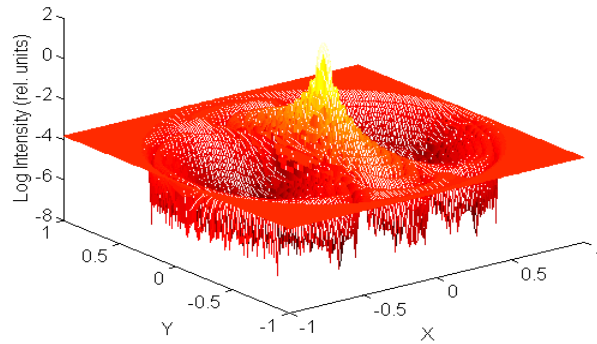
Figure 5: Planar grids of the angular distribution of the scattered light resulting from T-matrix computations of prolate spheroids, employing parallel polarization of the incident light with a zenith incident angle of 90° and a wavelength of 940 nm are presented. The intensity is presented on a logarithmic scale (base 10) and arbitrary units. The results of Prolate I are shown in (a) with a log intensity of the forward and back scattering of 1.72 and 4.31 (relative units), of Prolate II in (b) with corresponding values of 1.46 and -4.05 and finally of Prolate III in (c) with a log intensity of the forward and back scattering of 1.31 and -3.81.
