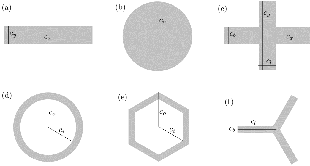
Figure 4: Examples of geometries for the waveguide: (a) Rectangular. (b) Circular. (c) Cross. (d) Annular. (e) Hexagonal. (f) Tripole.
