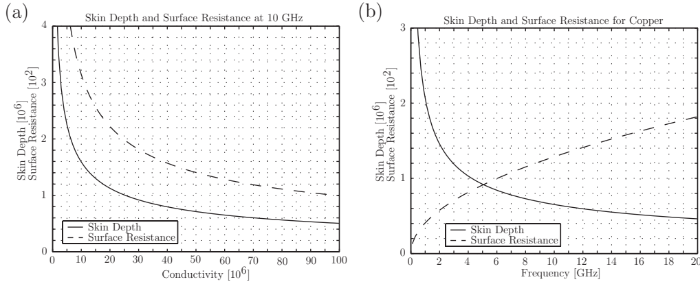
Figure 14: Skin depth, \delta , and surface resistance, R_s .
