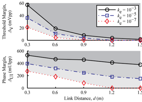
FIGURE 5. Measured eye margins for bit-error rates k_e < 10^{-3} , 10^{-5} , and 10^{-7} at 10 Gb/s data-rate, i.e. with a 100-ps UI. Both margins, i.e. threshold, \Delta_V , and phase, \Delta_{\phi} , are given peak-to-peak at the sampling point.
