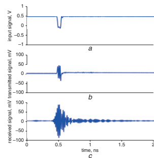
Fig. 2 Input signal of wavelet generator (Fig. 2a); on-chip measurement of generated signal (Fig. 2b) (centre frequency of wavelet is 59 GHz, de-embedded voltage swing is 177 mV pp ; pulse length of baseband signal is 53.9 ps, wavelet is 56.4 ps); received wavelet after transmission (Fig. 1c)
