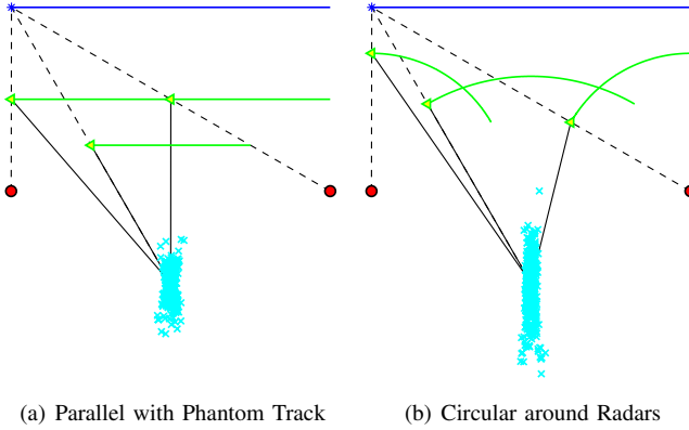
Fig. 4. Variance of Radar Position Estimates over Time for Different ECAV Trajectories but Identical Distributions of Measurement Noise
