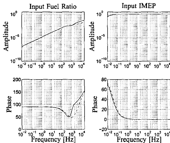
Fig. 15. Sensitivity functions for the transfer functions from fuel ratio and IMEP to \alpha_{50,p} (grey) and \alpha_{50,ion} (black), respectively.
