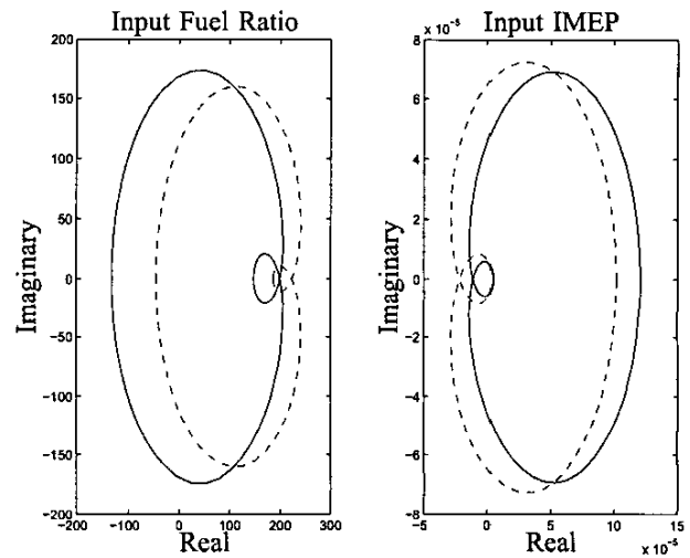
Fig. 13. Nyquist diagram ( left ) from fuel ratio to \alpha_{50,ion} ( solid ) and \alpha_{50,p} ( dashed ). Nyquist diagram ( right ) showing from IMEP to \alpha_{50,ion} ( solid ) and \alpha_{50,p} ( dashed ).
