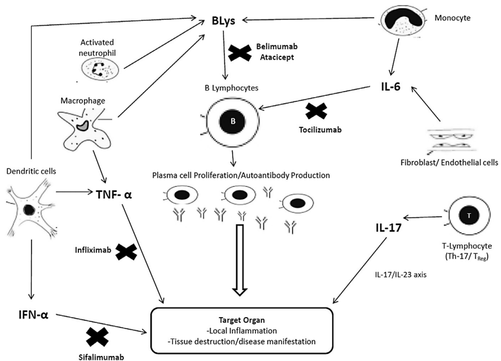
Schematic diagram to illustrate the complex interaction of different cytokines/immune cells and the rationale of anti-cytokine therapies.
