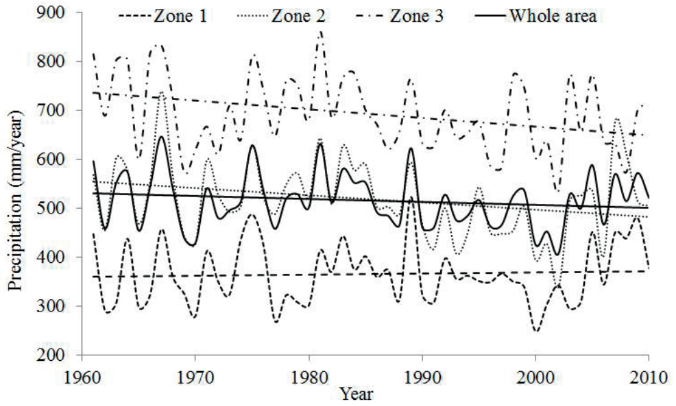
426 Fig. 3 Annual precipitation from 1961 to 2010 for the three different zones and the whole 427 area in the source region of the Yellow River
