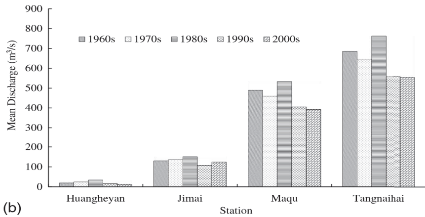
Fig. 4.3 (a) Annual and (b) decadal mean discharge at the four discharge stations
