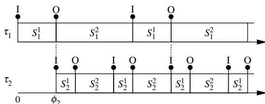
Figure 7 Segment layout in the cascaded PID controller. Task \tau_2 is given a phase \phi_2 = l_1^1 such that the value written by S_1^1 is immediately read by S_2^1 .
