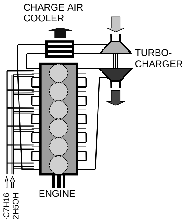
Figure 1 Engine system.
