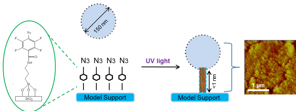
Figure 3.2. Schematic of the process used for the immobilization of MIP nanoparticles. Adapted from Paper 1 .
