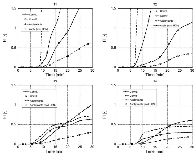
Figure 4-5 Fraction of an incapacitation dose for convective heat exposure compared with asphyxiant gases for the four tests in the Runehammar tunnel.
