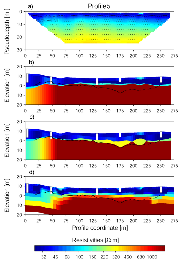
Figure 36 a) Apparent resistivity pseudo sections for profile 5. Resistivity models from: b) 2D-LCI; c) 2D-LCI with layer interfaces from the refraction seismic model as a priori information; d) 2D smooth inversion.
