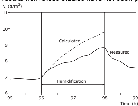
Figure 1. Comparison between measured indoor vapor content (solid line) and calculated indoor vapor content without taking moisture buffering into account (dashed line) for a house in Southern Sweden subjected to humidification by a humidifier.
