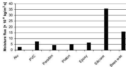
Figure 6. Moisture fluxes in the tested sealants.
