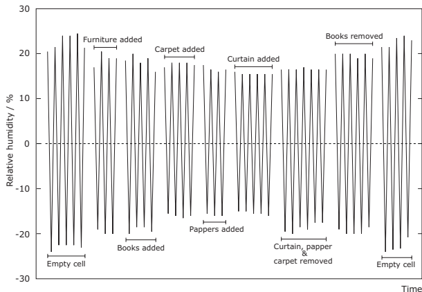
Figure VII. The moisture buffering effect of furniture and furnishings.
