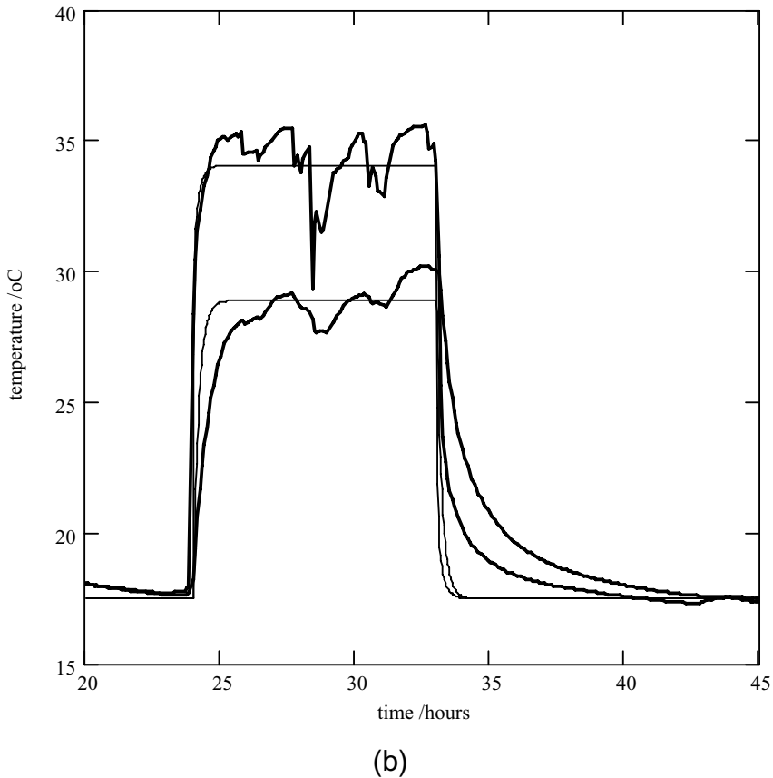
Figure 12. Thermal conditions for bed A (a) and B (b) measured and simulated for both bed systems. One sleeping cycle of 24 hours is shown. Measured temperatures are drawn with thick solid lines – the upper line representing the sensor on top of the mattress and the lower the sensor under the mattress (both in the torso region). The thin solid lines are the temperatures calculated with the proposed mathematical simulation model.
