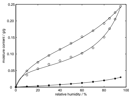
Figure V. Sorption isotherms for the wool fabric (above) and polyether foam (below) for the studied chair seat.
