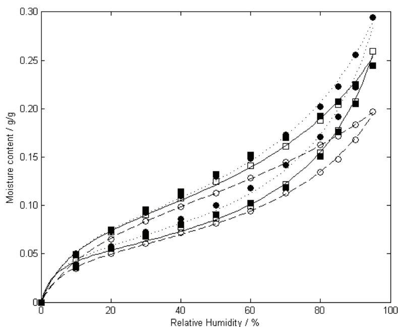
Figure 6. The sorption isotherms for the wool based fabrics: (○), 15% polyamide – 85% wool, (●) 50% viscose – 50% wool, (□) 100% felted wool and (■) 100% plain wool . The Hailwood-Horrobin sorption isotherms are shown with solid line for the felted wool fabric, dashed line for the polyamide-wool fabric and dotted line for the viscose-wool fabric.
