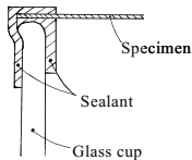
Figure 4. Cup design used for thin test samples
