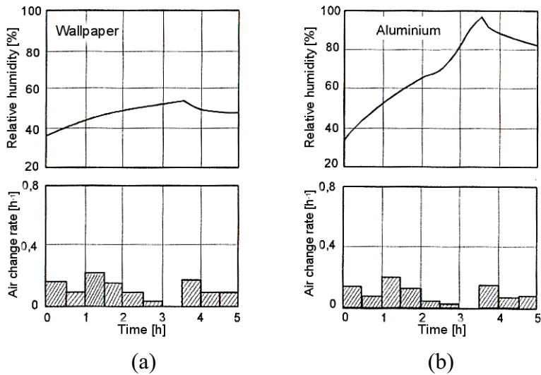
Figure 4. a: Test room with wallpaper. b. Reference room with aluminium panels. At the top is the RH in the test rooms shown during the moisture production of 700 g/h during 3.5 hours. In the bottom are the air change rates in the test rooms, which were influenced by the outdoor conditions.
