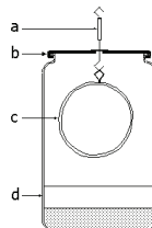
Figure 7. Experimental set-up for the JAR-method. a) The hook trough the lid enabling gravimetric determination with sample in desired climate. b) The vapor-tight lid. c) The sample. d) The saturated salt solution used for generating desired RH.
