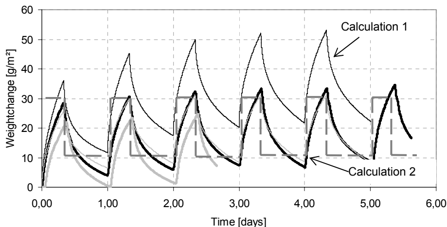
Figure 4. The MBV practical test method. The dashed grey line shows the variations in RH - 8 h at 75% RH and 16 h at 33% RH. The solid grey lines represent measurements for spruce plywood performed with this mode. The black lines represent two calculations of moisture buffering using material properties determined under steady state conditions. Calculation 1 uses the moisture capacity dw/d\phi taken from the sorption isotherm and calculation 2 uses a moisture capacity dw/d\phi half the size of the one used in calculation 1. Calculation 2 will therefore use a moisture capacity dw/d\phi that is closer to the one of a scanning curve. The curve for calculation 2 coincides to a high extent with one of the measurements (thin grey line).
