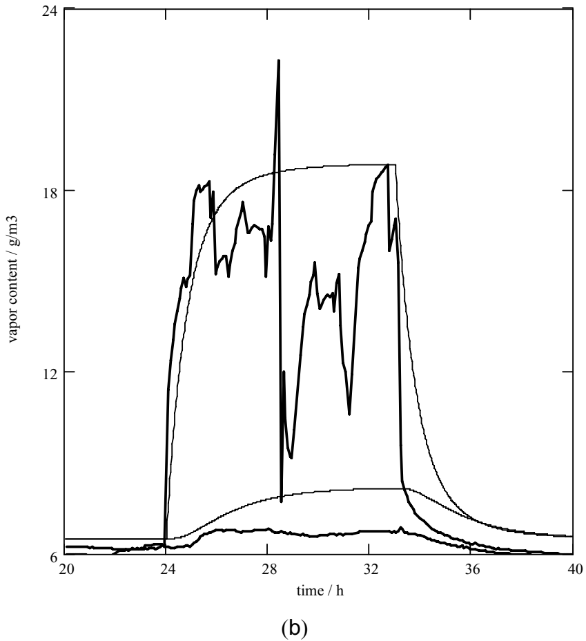
Figure 13. Moisture conditions for bed A (a) and bed B (b) measured and simulated for both bed systems. One sleeping cycle of 24 hours is shown. Measured temperatures are drawn with thick solid lines – the upper line representing the sensor on top of the mattress and the lower the sensor under the mattress (both in the torso region). The thin solid lines are the vapor contents calculated with the basic mathematical simulation model.
