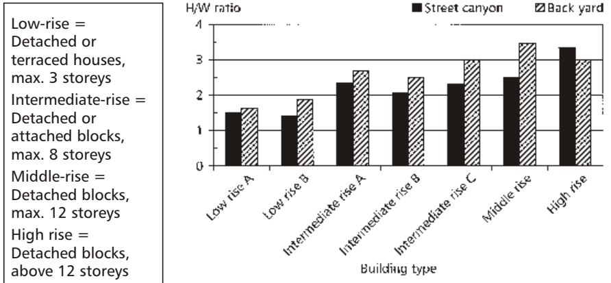
Fig. 6.24 The maximum H/W ratios of the street canyons and back yards permitted for different building types in Colombo. (Calculated from UDA (1999b). There is no maximum height limit for high-rise buildings. Here, the height has been assumed to be 60 m).
