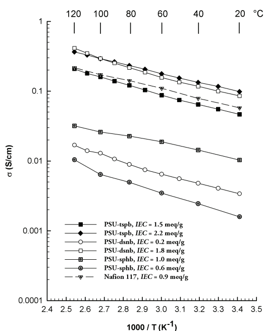
Figure 11. Arrhenius plots of proton conductivity data measured by electrochemical impedance spectroscopy with membranes immersed in water.
