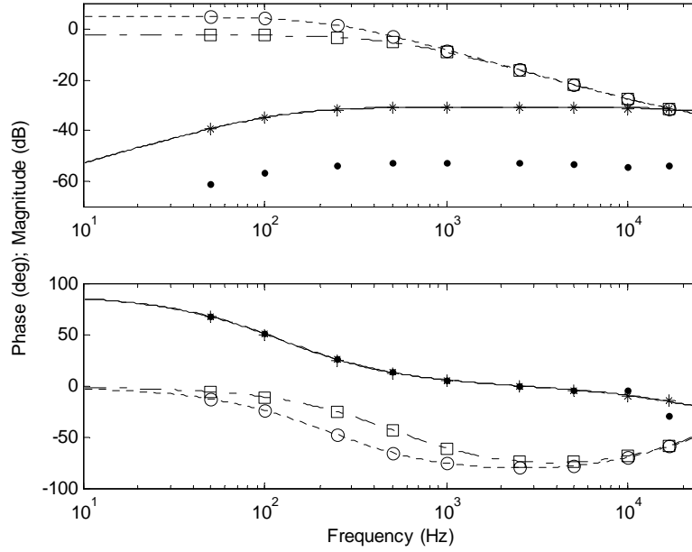
Figure 7.13: The output impedance of a buck converter controlled by (7.21). Dash-dotted line ( \square ): H_i(s)=0 and R=R_{\min} . Dotted line (O): H_i(s)=0 and R=R_{\max} . Solid line (+): H_i(s)=1 and R=R_{\min} . Dashed line (x): H_i(s)=1 and R=R_{\max} . Note that the two last mentioned lines almost coincide. Points: Simulation with R=R_{\max} and H_i(s) equal to 1/F_h(s) in series with a second order filter.
