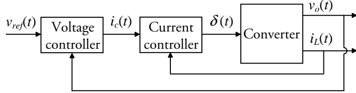
Figure 3.1: Current-mode control.
