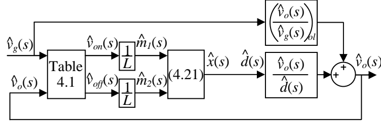
Figure 4.12: A model of the audio susceptibility.
