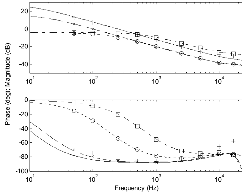
Figure 7.29: The audio susceptibility of a buck-boost converter controlled by (7.21). Dash-dotted line ( \square ): H_i(s)=0 and R=R_{\min} . Dotted line ( \circ ): H_i(s)=0 and R=R_{\max} . Solid line ( + ): H_i(s)=(1+D)/D' and R=R_{\min} . Dashed line ( \times ): H_i(s)=(1+D)/D' and R=R_{\max} .
