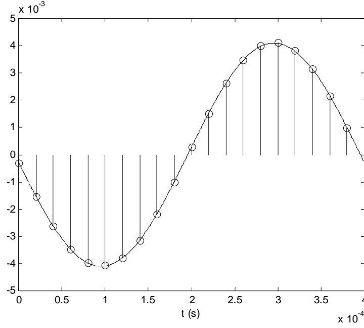
Figure 4.8: The sinusoidal signal corresponding to the coefficient c(1) together with the \hat{d}(n) ( \omega_m = 5000\pi rad/s).
