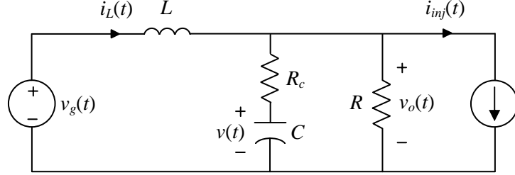
Figure 2.3: The circuit of the buck converter during t_{on} .
