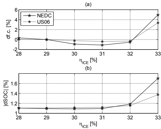
Figure 4.6 Relative change in fuel consumption (a), with regard to the fuel consumption obtained with \eta_{ICE_{eff}} equal to 29%. Mean SOC deviation (b) with respect to the reference value of 70%.
