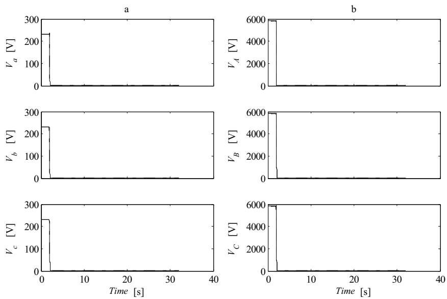
Figure A1.6.8 Phase a-b fault. a) Phase voltages at induction generator terminals b) Phase voltages on the high voltage side of step up transformer. l_{L1} = 2 km (solid lines) and l_{L1} = 6 km (dashed lines). P_{load} = 5 kW, R_f = 0 \Omega
