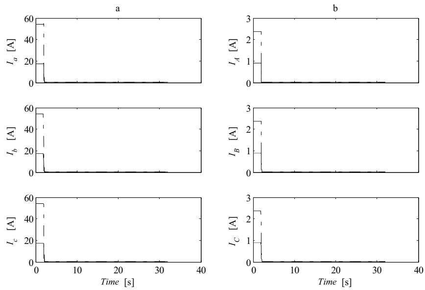
Figure A1.6.7 Phase a-b fault. a) Phase currents at induction generator terminals b) Phase currents on the high voltage side of step up transformer. l_{L1} = 2 km (solid lines) and l_{L1} = 6 km (dashed lines). P_{load} = 5 kW, R_f = 0 \Omega
