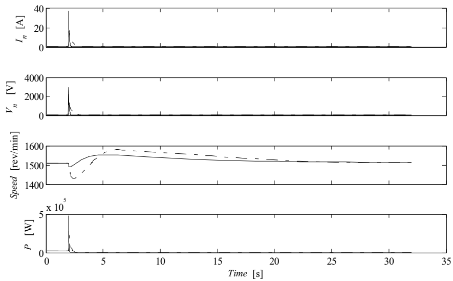
Figure A1.4.3 Phase A-B fault. Negative sequence current and voltage at fault point, generator speed, generator active power. R_f = 0 \Omega (solid lines) and R_f = 200 \Omega (dashed lines). l_{L1} = 4 \text{ km} , P_{load} = 5 \text{ kW}
