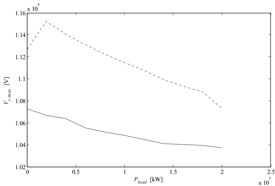
Figure 4.5 Maximum voltage V_C on the 10 kV side after a Phase A to earth fault, excluding the fast pos- fault transient. l_{L1} = 4 km (solid line) and l_{L1} = 10 km (dashed line).
