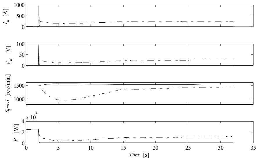
Figure A1.6.3 Phase a-b fault. Negative sequence current and voltage at fault point, generator speed, generator active power. R_f = 0 \Omega (solid lines) and R_f = 0,6 \Omega (dashed lines). l_{L1} = 4 \text{ km} , P_{load} = 5 \text{ kW}
